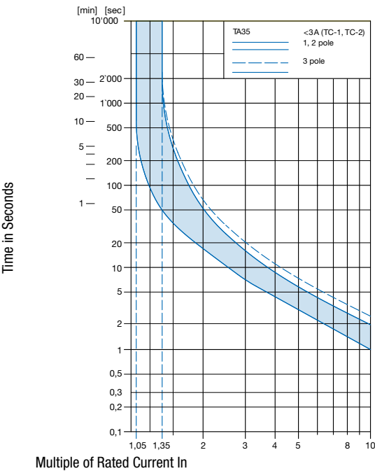
Reference Temperature +23°
