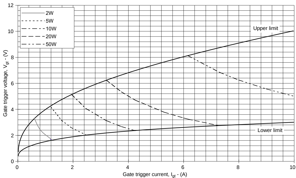
Fig.8 Gate characteristics
