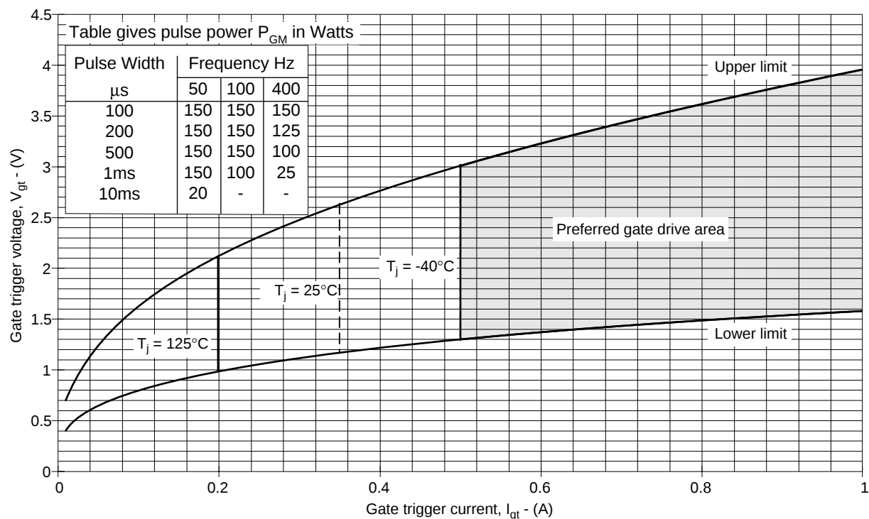
Fig.7 Gate characteristics
