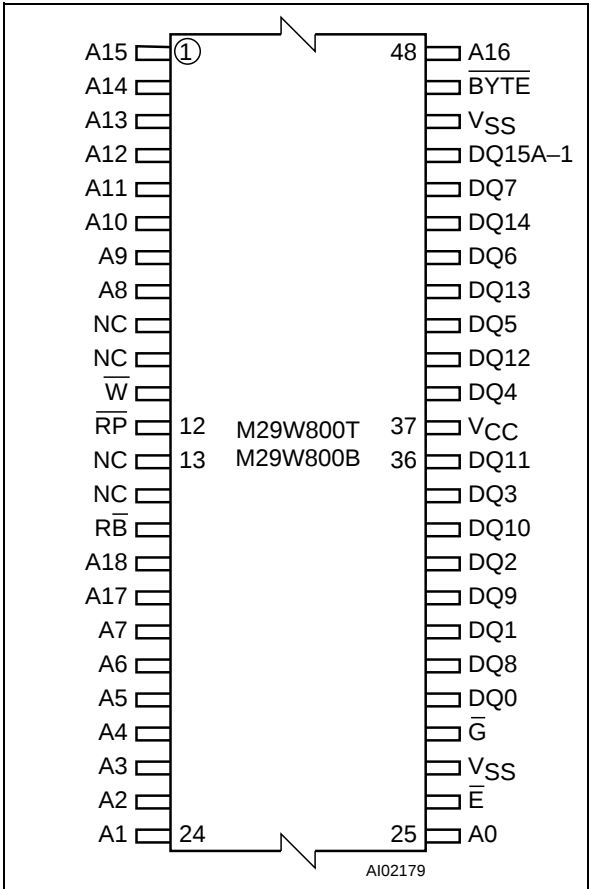
Figure 3. TSOP Connections
