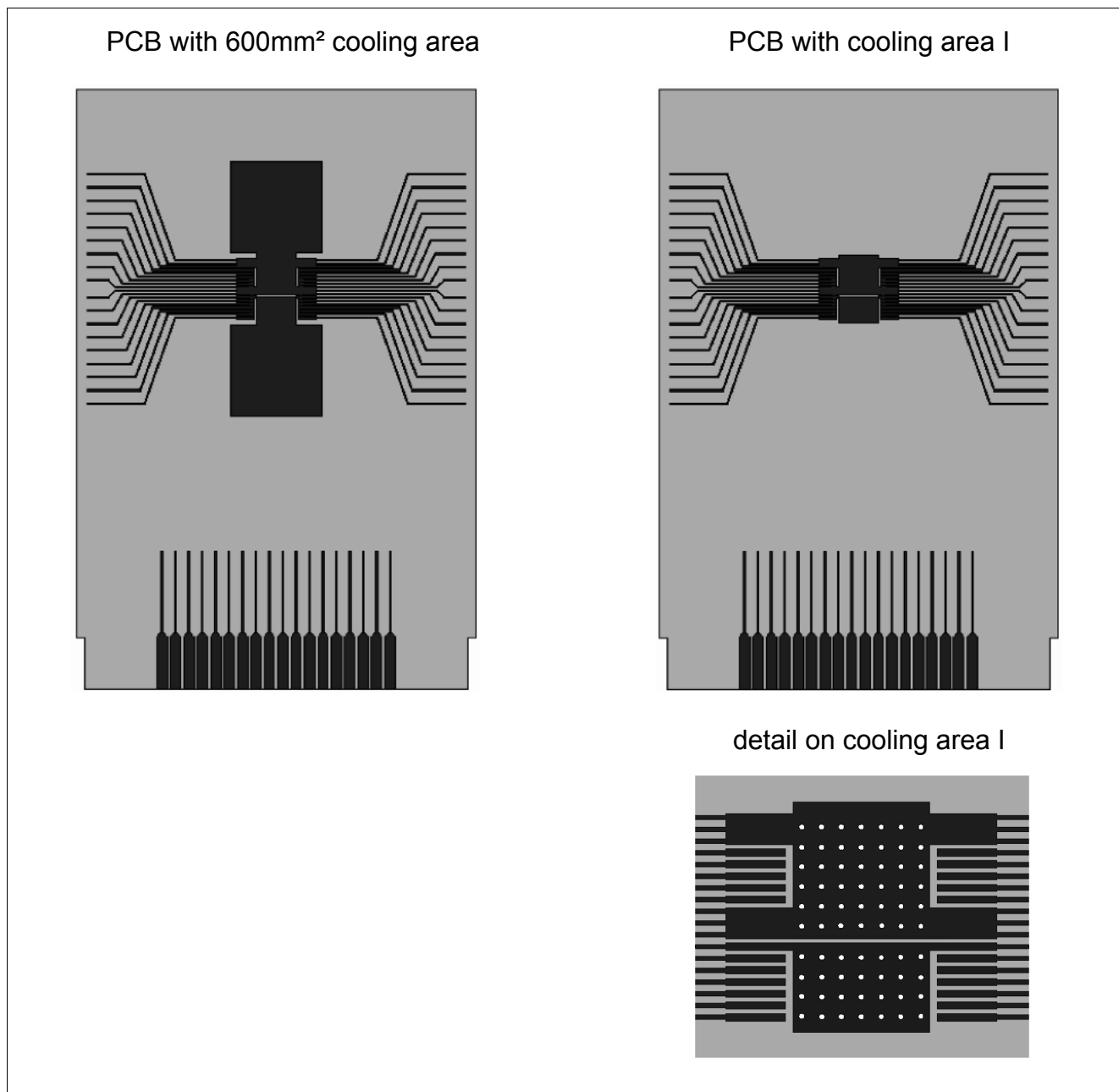
Figure 7 Top view of PCB with different cooling areas used for ZthJA simulation
