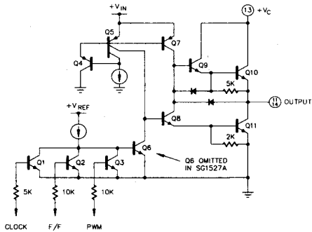
FIGURE 6-OUTPUT CIRCUIT (1/2 Circuit Shown)
