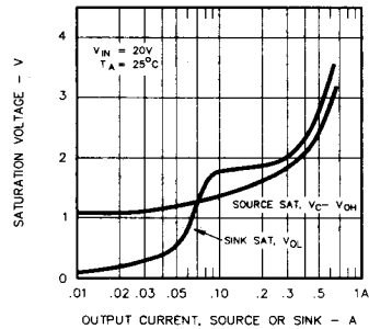
FIGURE 7-OUTPUT SATURATION CHARACTERISTICS
