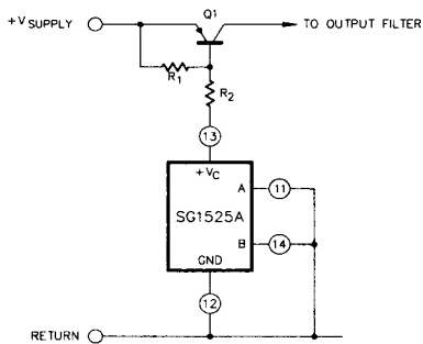
FIGURE 6-OUTPUT CIRCUIT (1/2 Circuit Shown)
