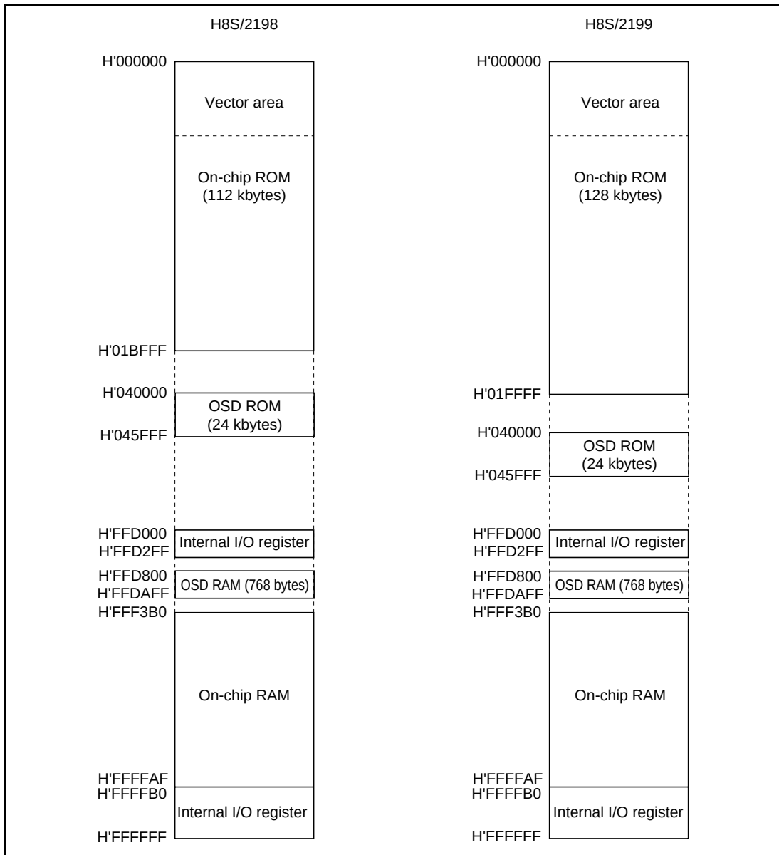
Figure 3.2 Address Map (2)
