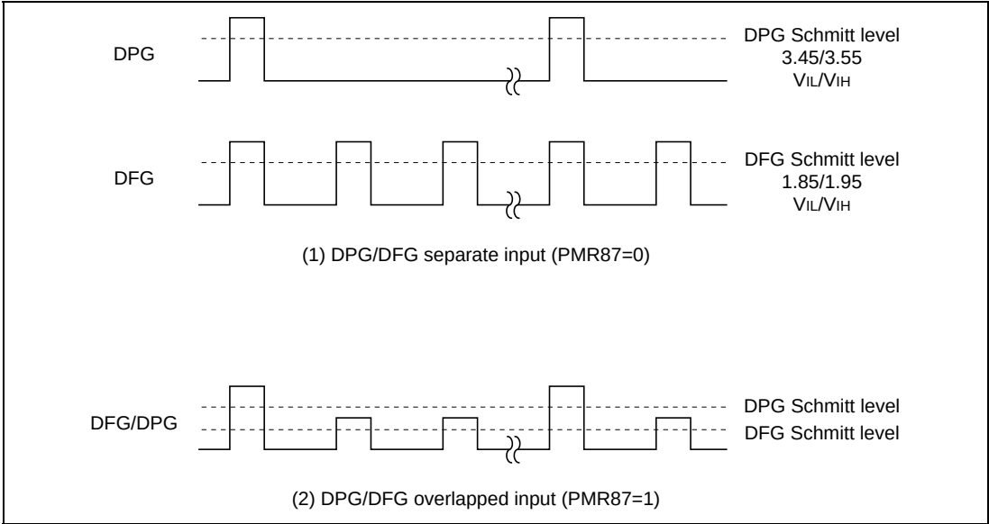
Figure 26.5 DFG/DPG Input Signals
