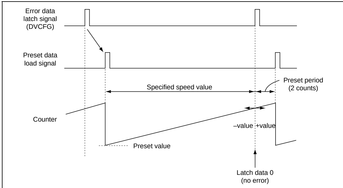
Figure 26.33 Example of the Capstan Speed Error Detection
