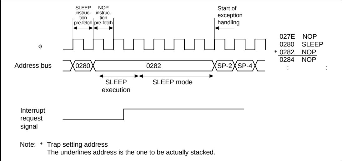
Figure 25.18 SLEEP Instruction (3)
