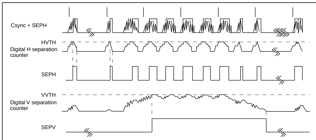
Figure 27.9 VVTHR Value and SEPV Generation Timing When Digital LPF Is Enabled
