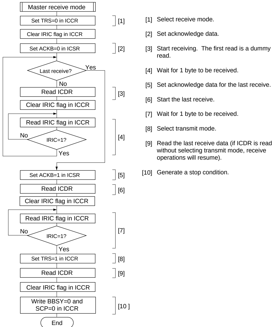
Figure 23.15 Flowchart for Master Receive Mode (Example)
