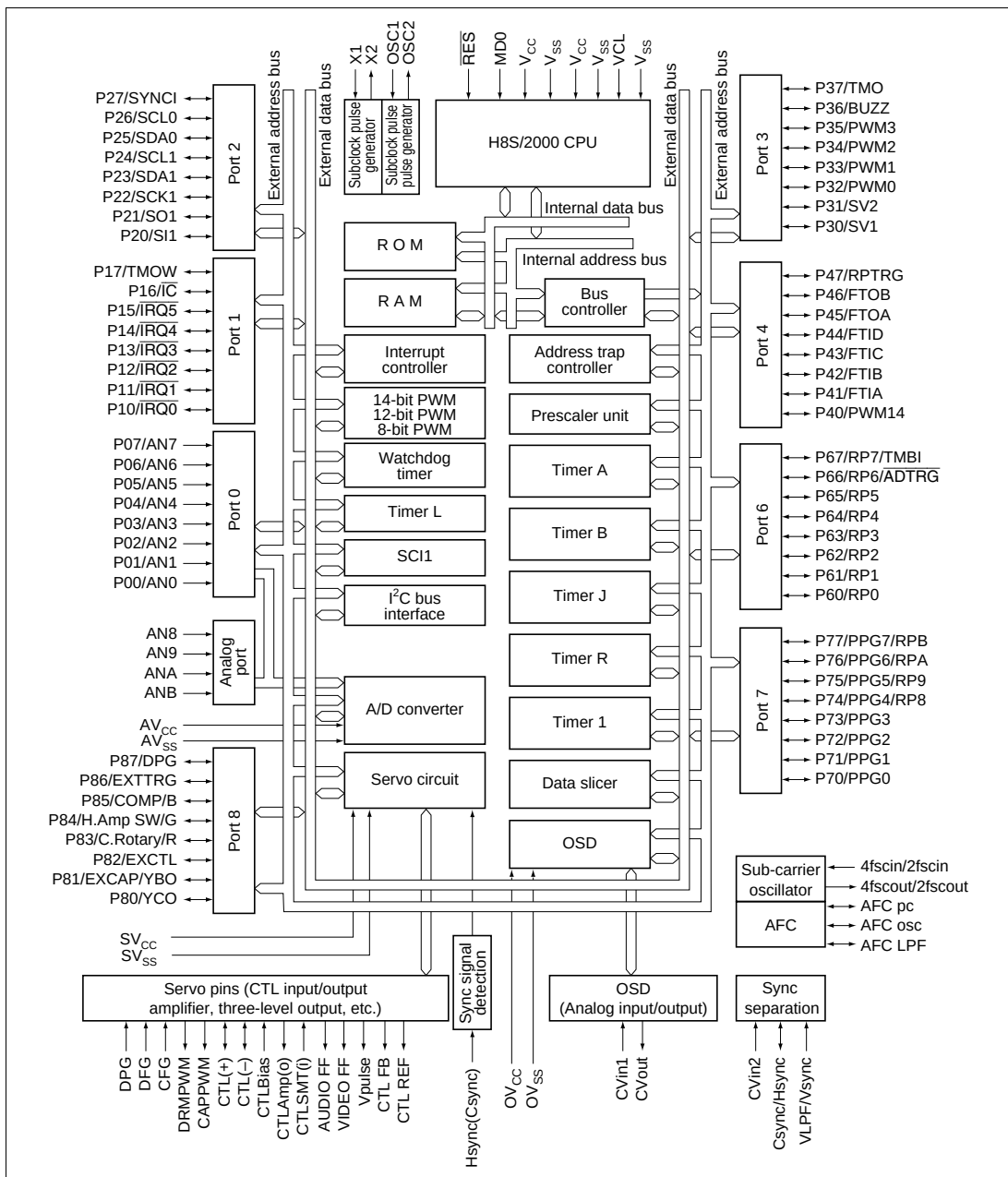
Figure 1.1 Internal Block Diagram of H8S/2199 Series
