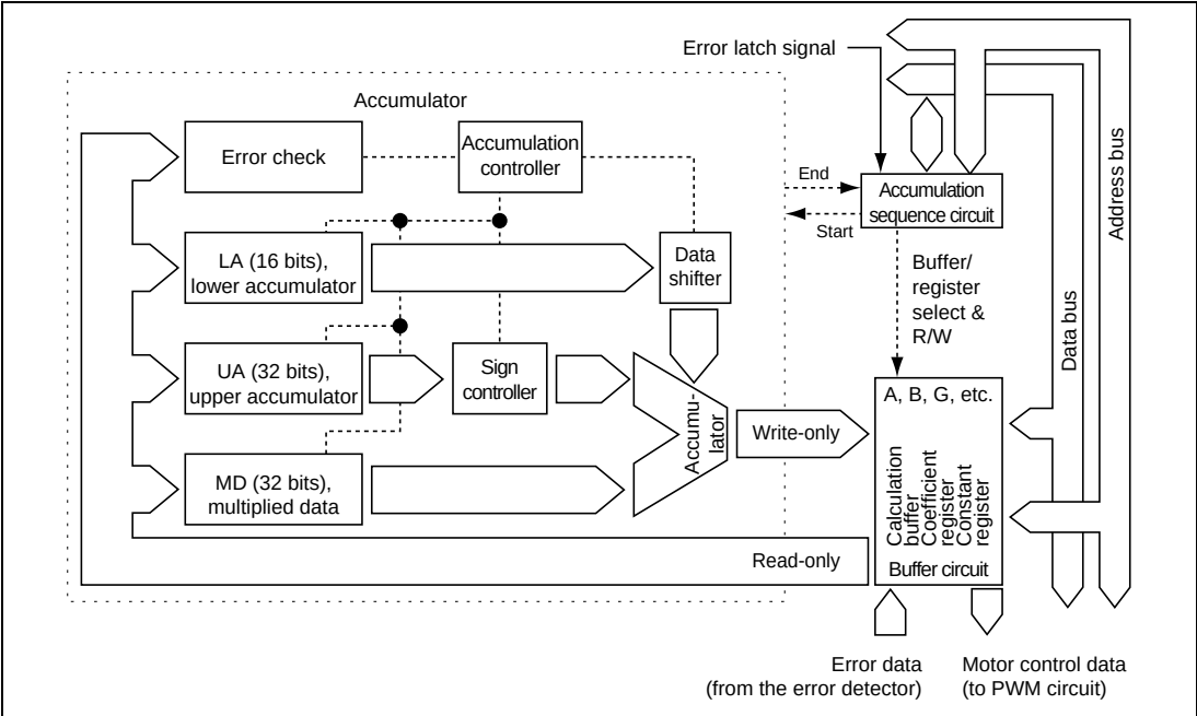
Figure 26.38 Block Diagram of Digital Filter Circuit
