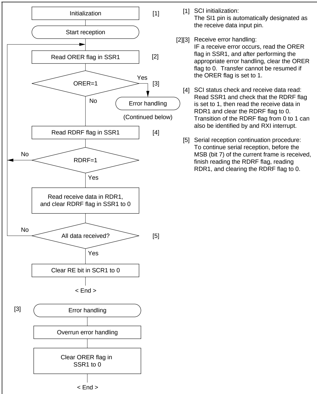
Figure 22.20 Sample Serial Reception Flowchart
