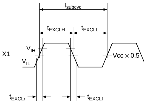
Figure 30.11 Subclock Input Timing
