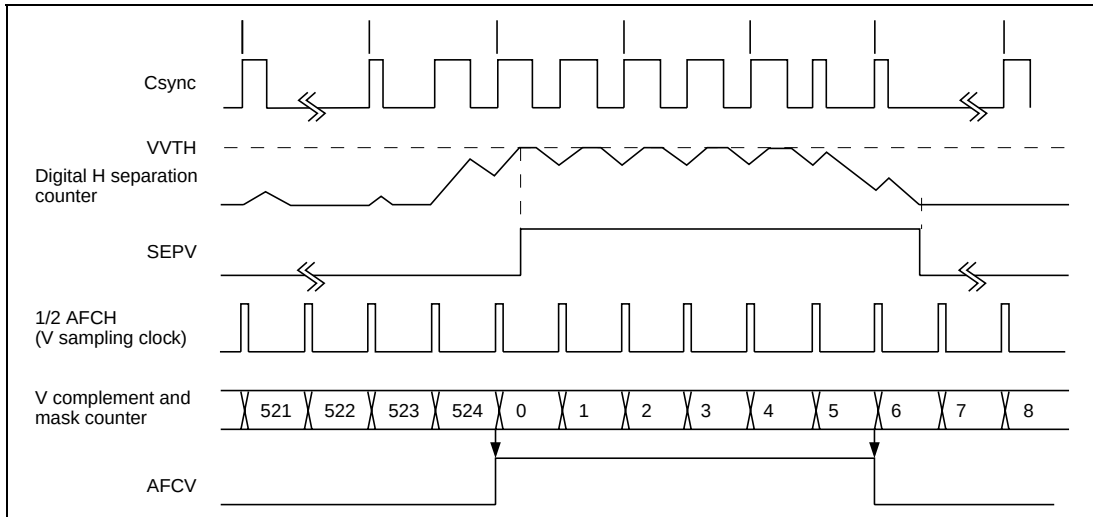
Figure 27.10 AFCV Generation Timing When V Complement Function Is Enabled (for NTSC)
