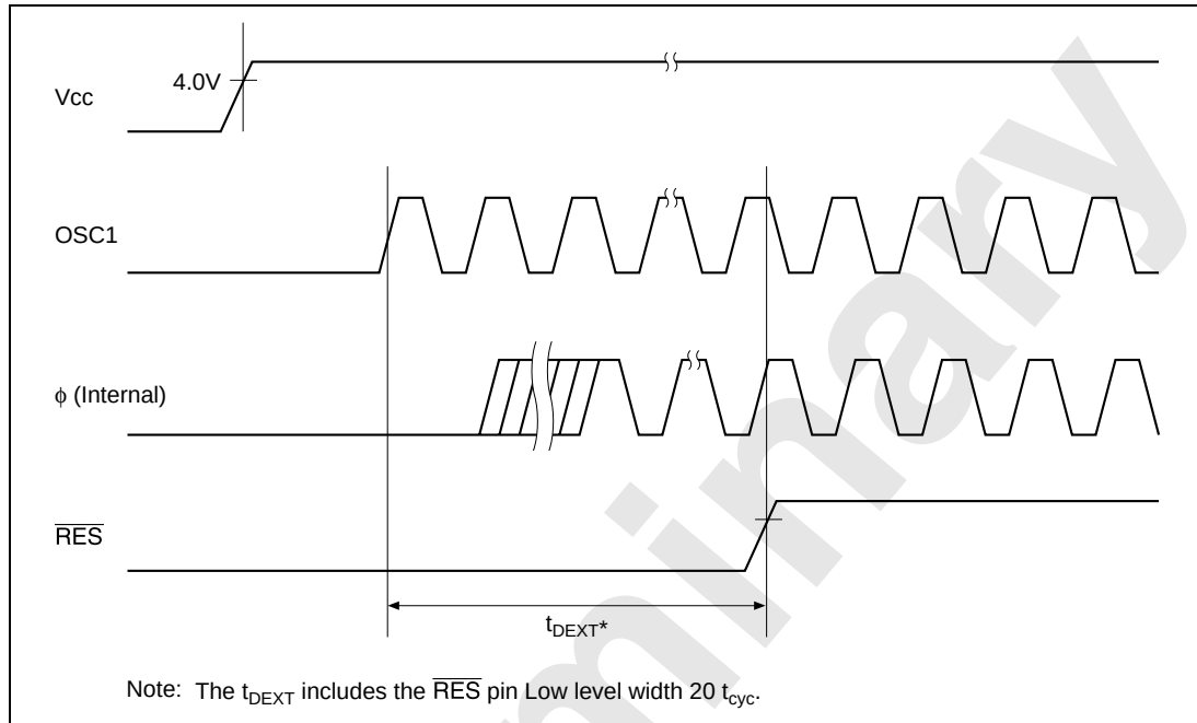
Figure 30.3 External Clock Stabilization Delay Timing
