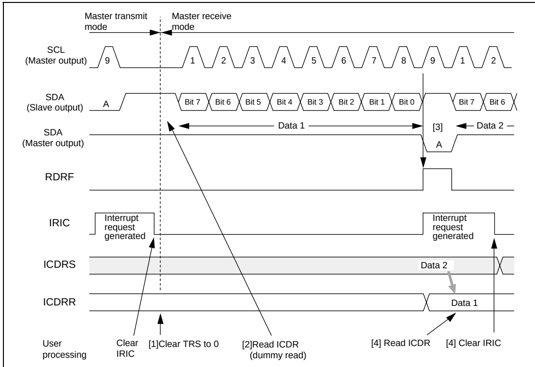
Figure 23.8 Example of Timing in Master Receive Mode (MLS = WAIT = ACKB = 0)
