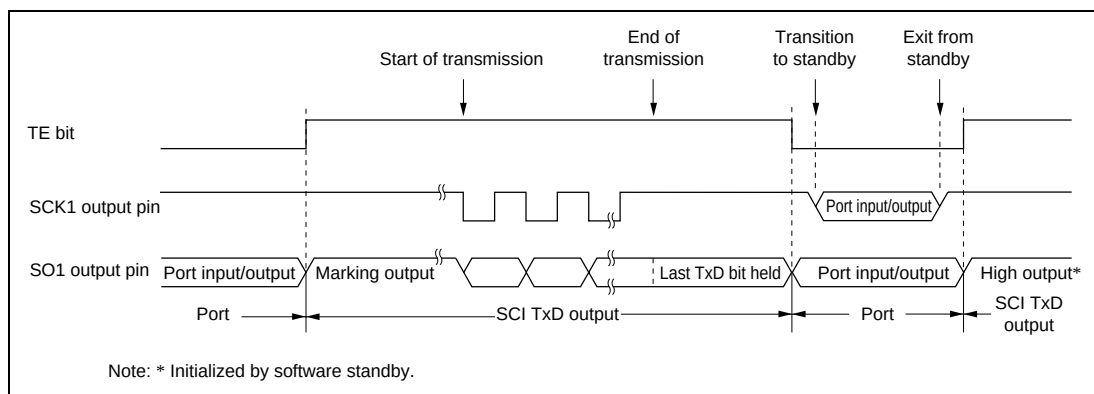
Figure 22.26 Synchronous Transmission Using Internal Clock
