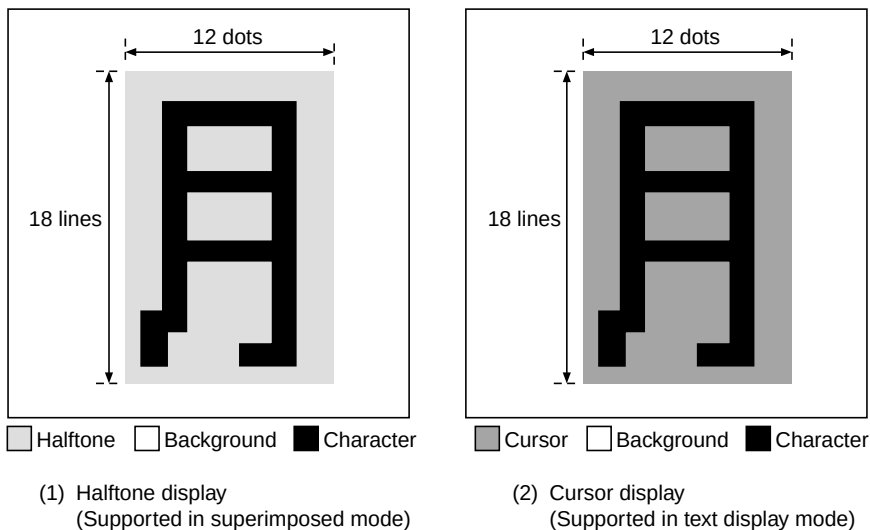
Figure 29.5 Halftone and Cursor Display Examples
