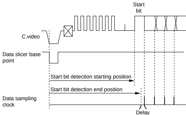
Figure 28.6 Data Sampling Clock When Start Bit is not Detected
