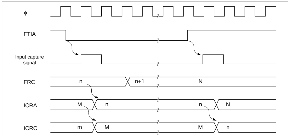
Figure 16.8 Input Capture Signal Inputting Timing Chart Under the Buffer Mode (under normal state)
