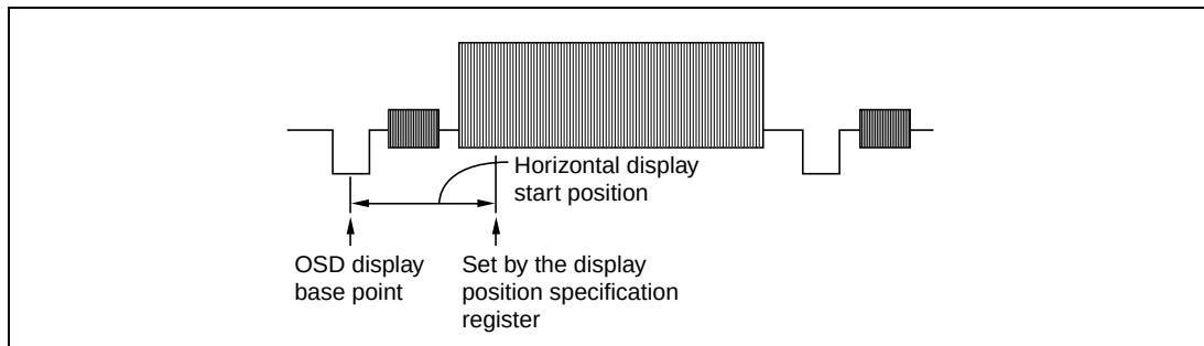
Figure 29.11 Base Point for Horizontal Display Start Position
