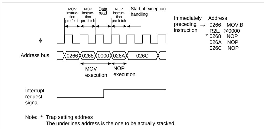
Figure 25.3 Basic Operations (2)
