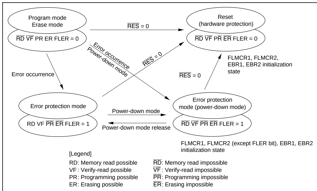
Figure 7.14 Flash Memory State Transitions
