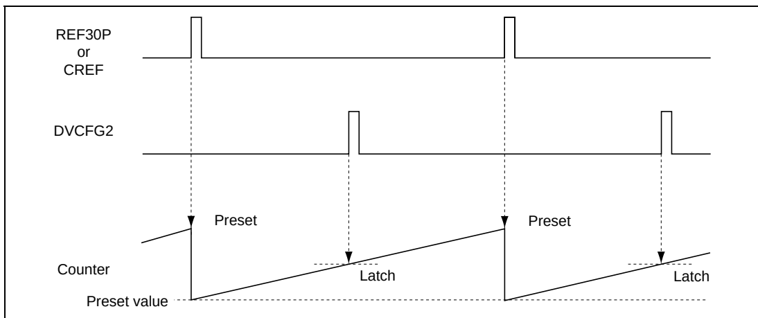
Figure 26.36 Capstan Phase Control in Record Mode
