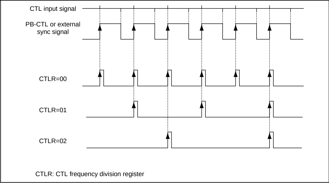
Figure 26.64 CTL Frequency Division Waveforms
