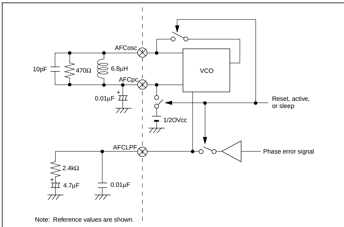
Figure 27.21 Circuit Example for a 576 x fh Reference Clock
