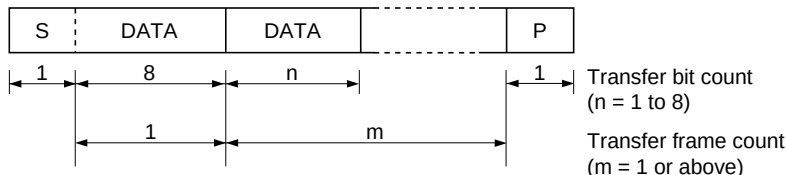
Figure 23.4 I²C Bus Data Format (Serial Format)
