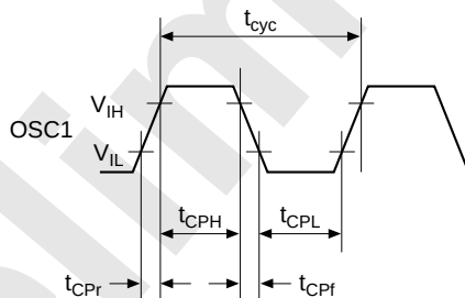
Figure 30.1 System Clock Timing
