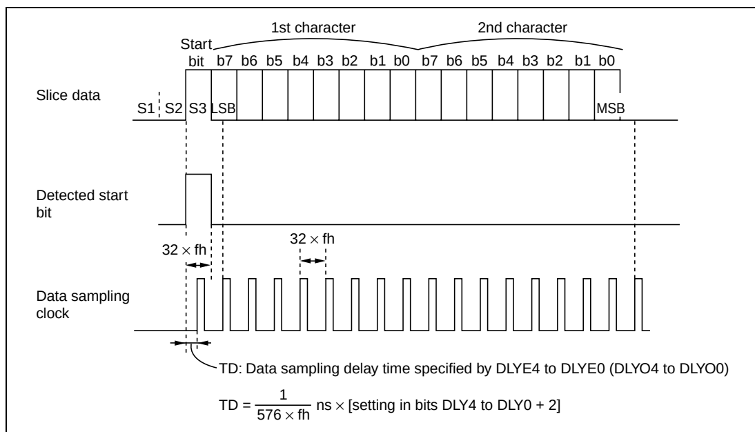
Figure 28.3 Data Sampling Clock Description
