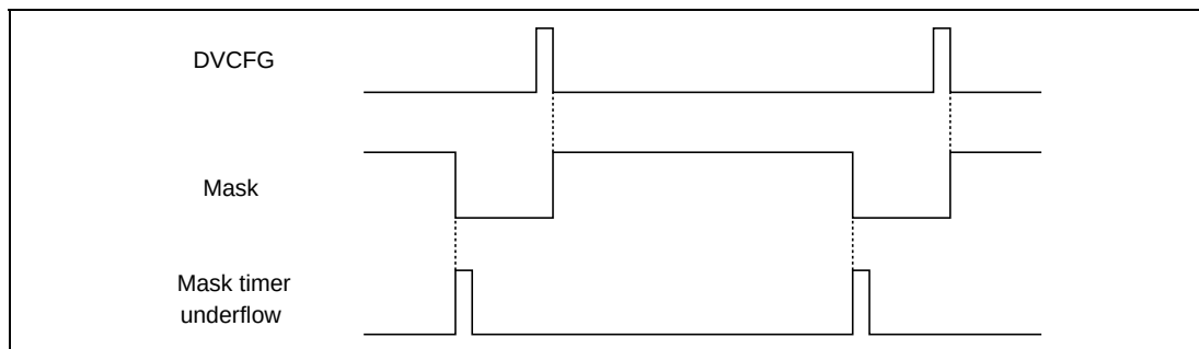
Figure 26.67 Mask Signal
