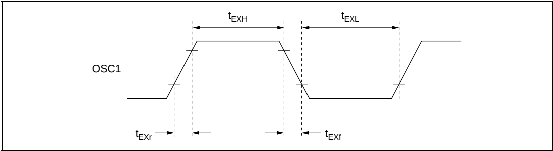
Figure 9.6 External Clock Input Timing
