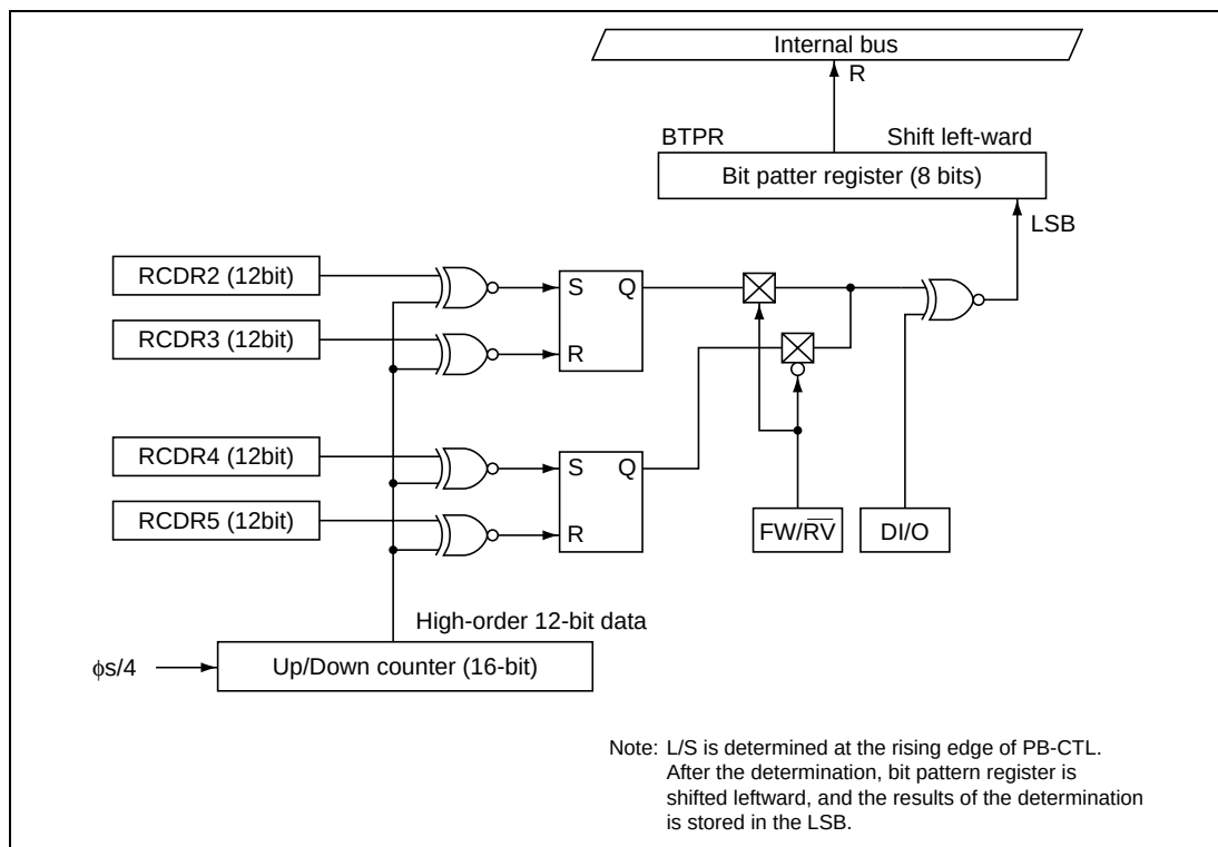
Figure 26.59 Detection of Long/Short Pulse
