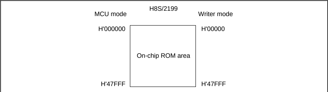
Figure 7.15 Memory Map in Writer Mode
