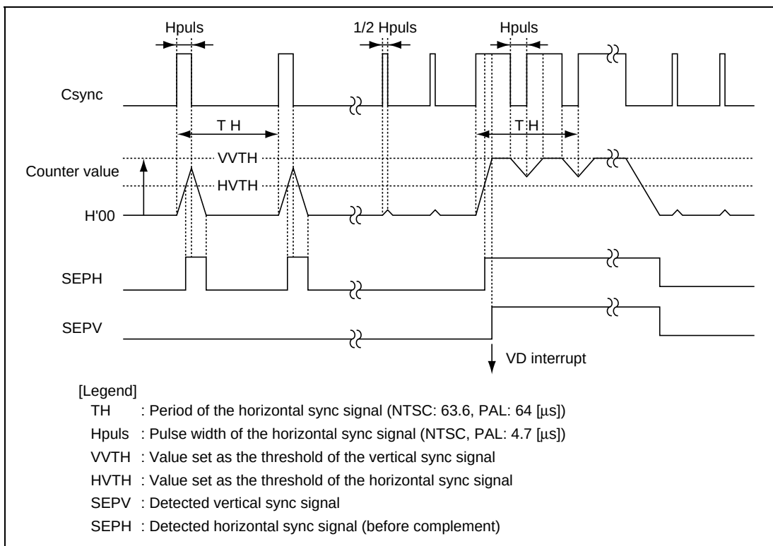
Figure 26.73 Threshold Values and Separated Sync Signals
