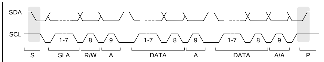
Figure 23.5 I²C Bus Timing
