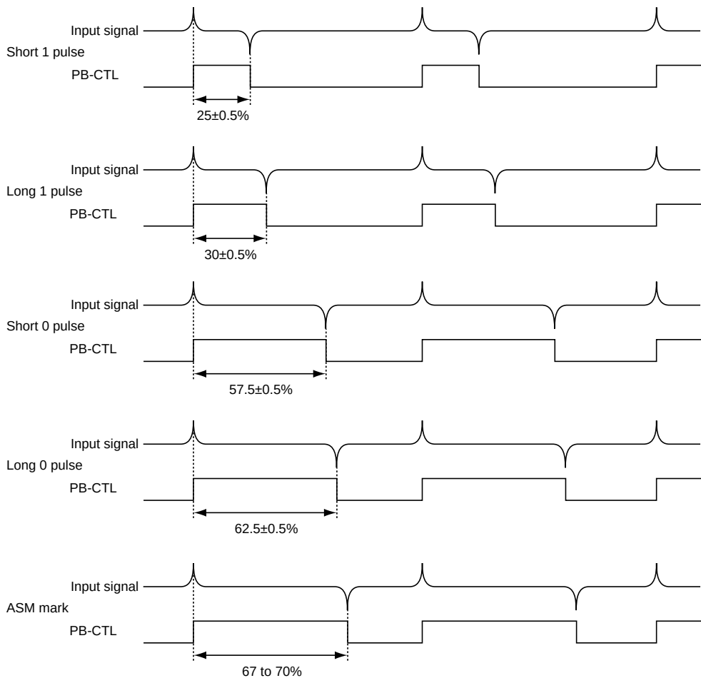
Figure 26.55 PB-CTL Signal Duty Cycle
