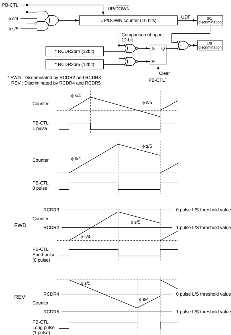
Figure 26.56 Duty Discriminator
