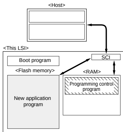
Figure 7.4 Boot Mode
