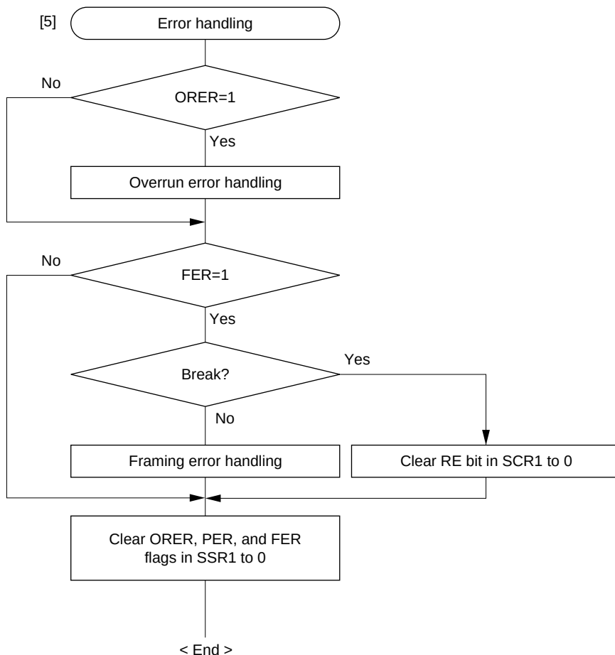
Figure 22.14 Sample Multiprocessor Serial Reception Flowchart (2)
