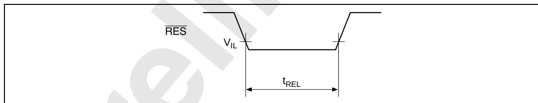
Figure 30.4 Reset Input Timing
