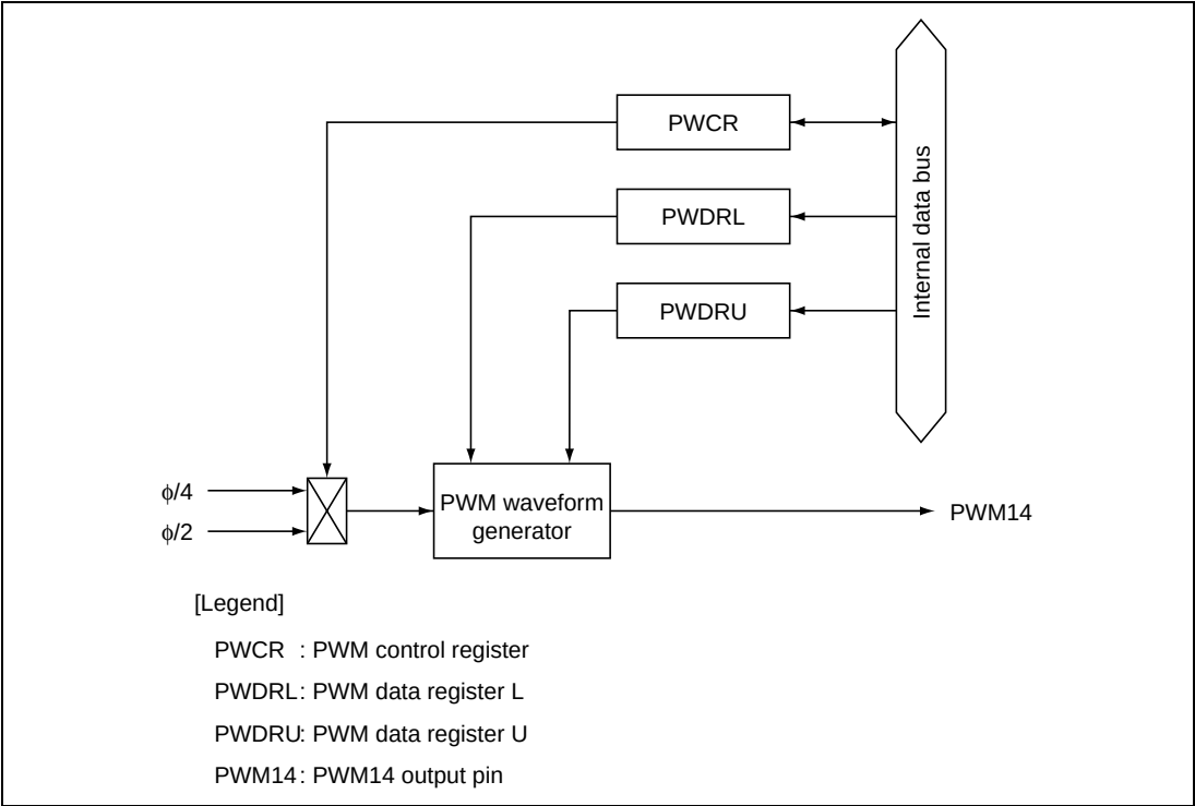
Figure 20.1 Block Diagram of 14-Bit PWM
