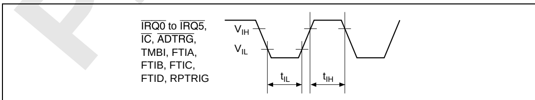
Figure 30.14 Input Timing
