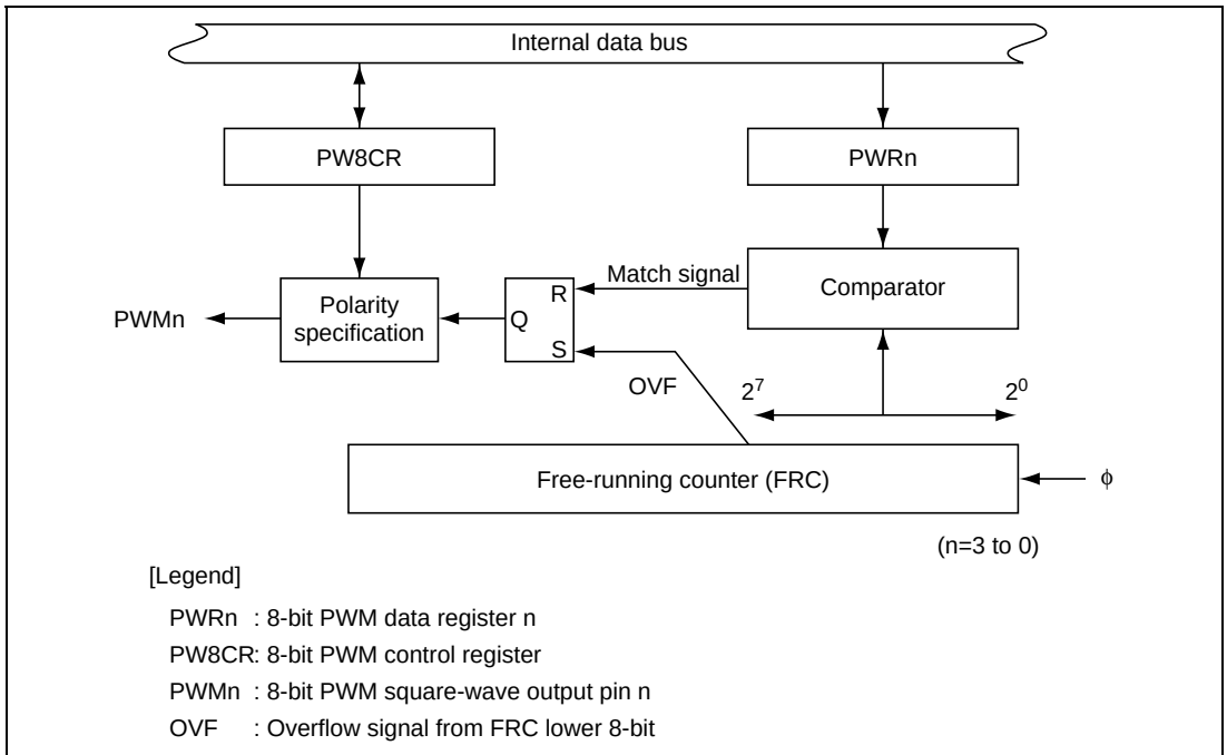
Figure 18.1 Block Diagram of 8-Bit PWM (1 channel)
