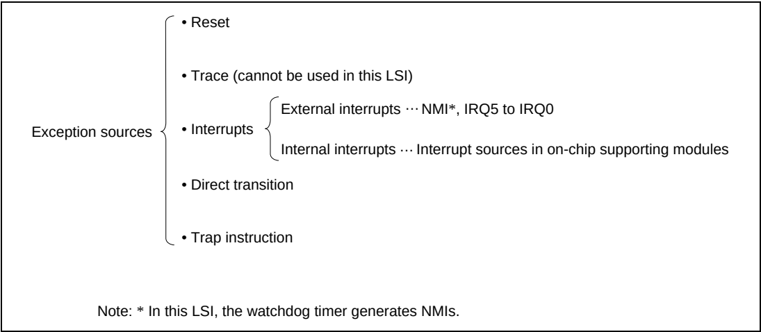
Figure 5.1 Exception Sources
