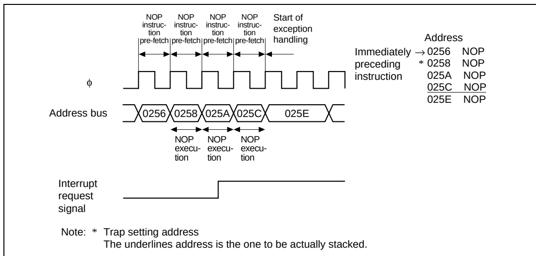
Figure 25.4 Basic Operations (3)
