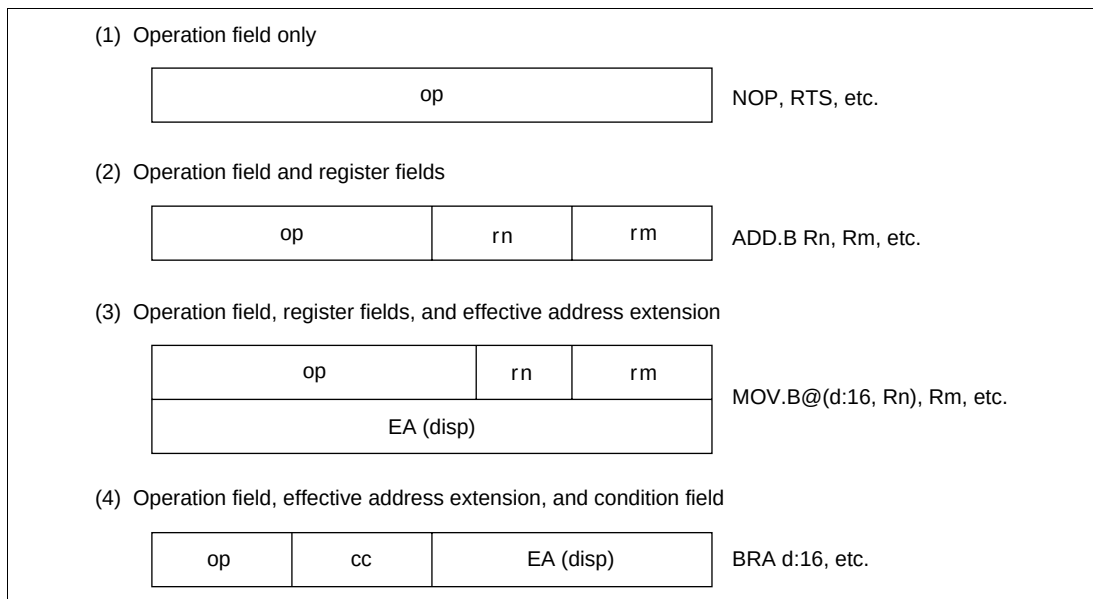
Figure 2.13 Instruction Formats (Examples)
