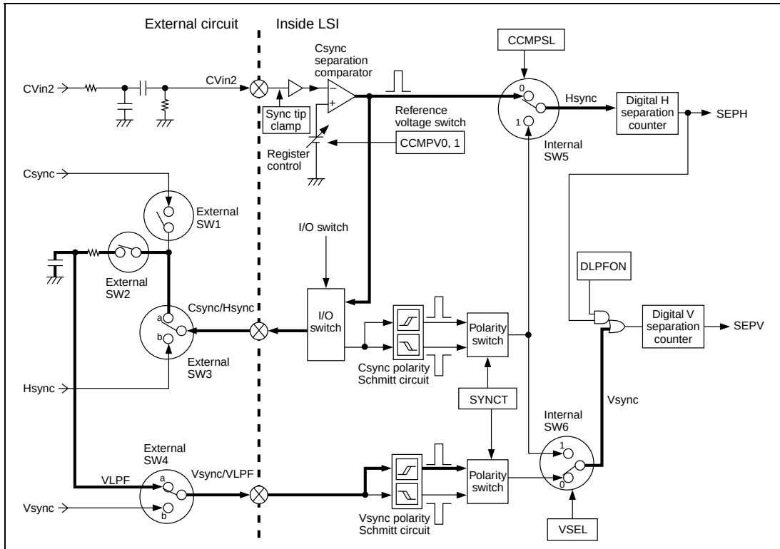
Figure 27.15 Sync Source Selection When Using the CVin2 Signal and the Vsync Schmitt Circuit
