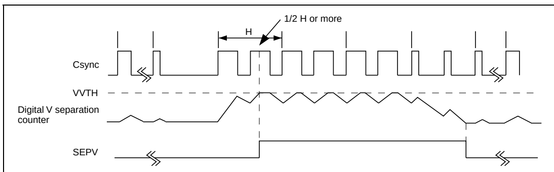
Figure 27.8 VVTHR Value and SEPV Generation Timing
