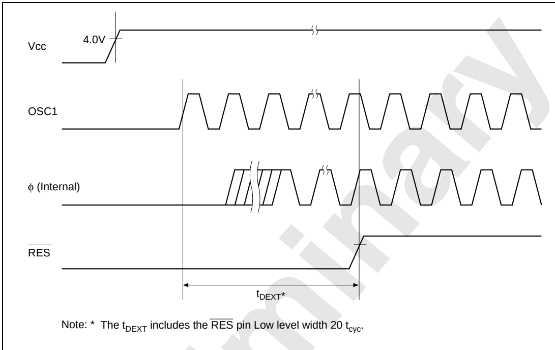
Figure 30.12 External Clock Stabilization Delay Timing
