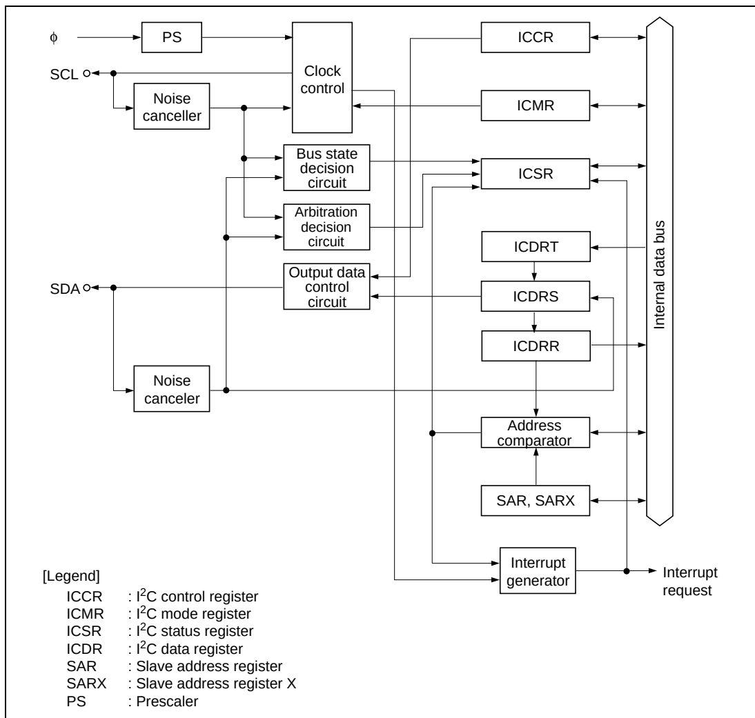
Figure 23.1 Block Diagram of I 2 C Bus Interface
