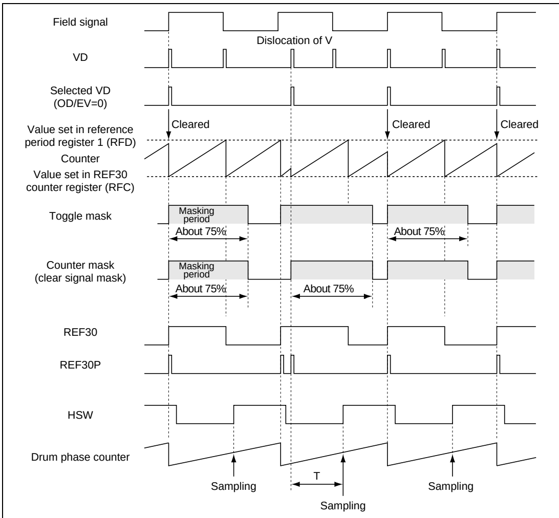
Figure 26.11 Generation of the Reference Signal when in REC (V Dislocated)
