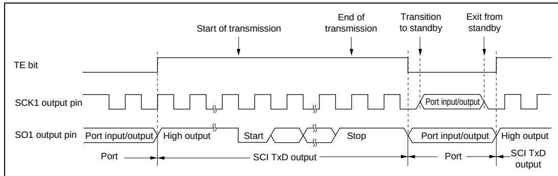
Figure 22.25 Asynchronous Transmission Using Internal Clock
