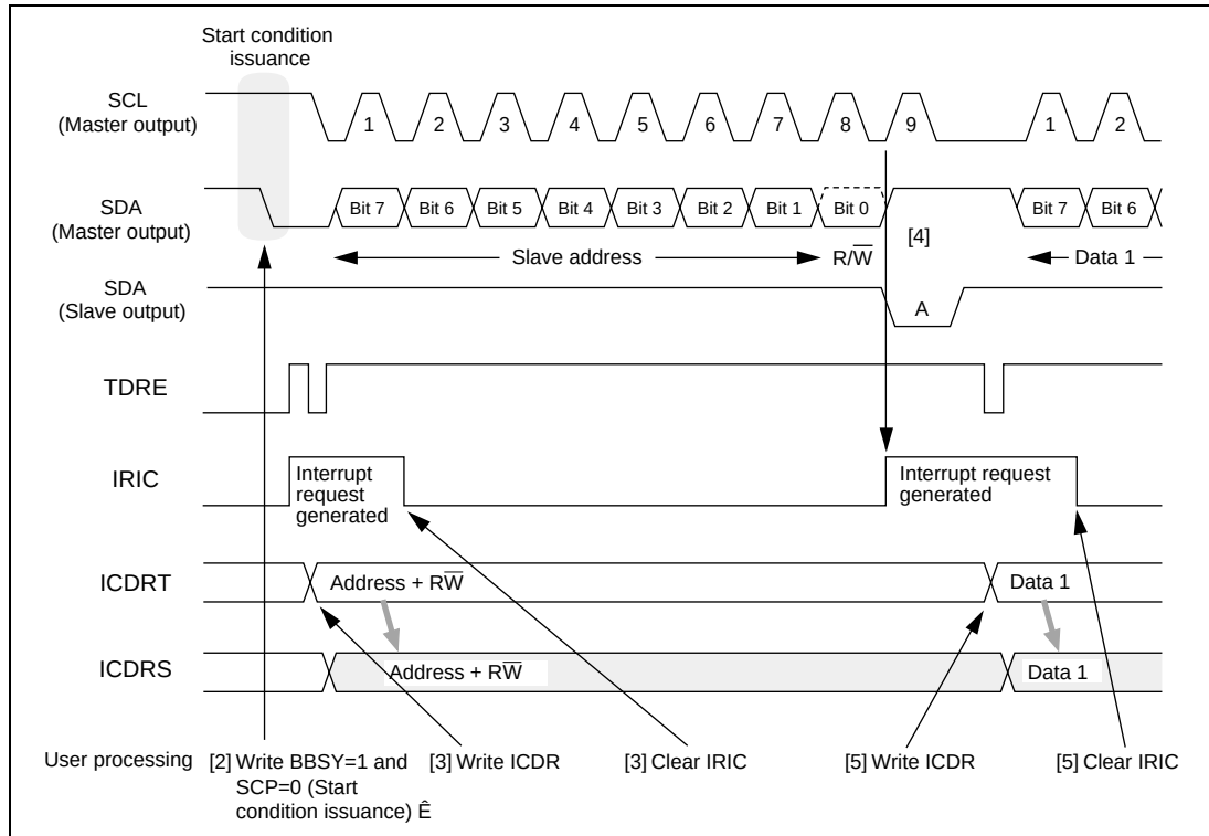
Figure 23.6 Example of Timing in Master Transmit Mode (MLS = WAIT = 0)
