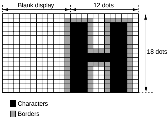
Figure 29.17 Border Neighboring a Blank Character (Example)
