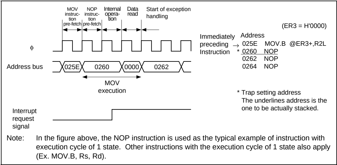
Figure 25.2 Basic Operations (1)
