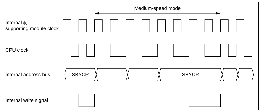
Figure 4.2 Medium-Speed Mode Transition and Clearance Timing
