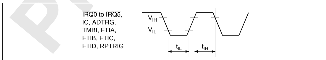
Figure 30.5 Input Timing
