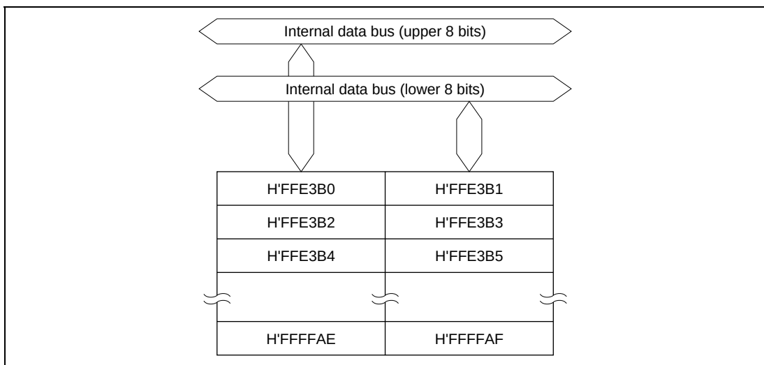
Figure 8.1 Block Diagram of RAM (H8S/2199)
