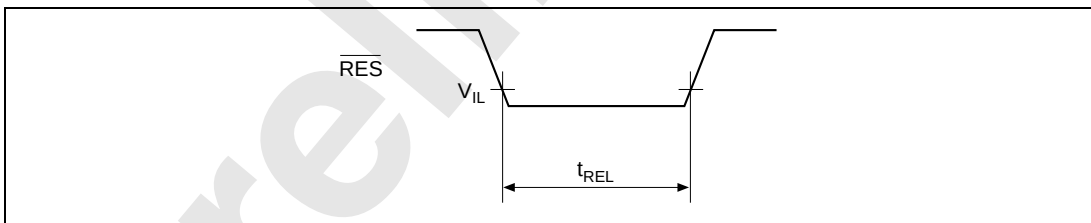
Figure 30.13 Reset Input Timing
