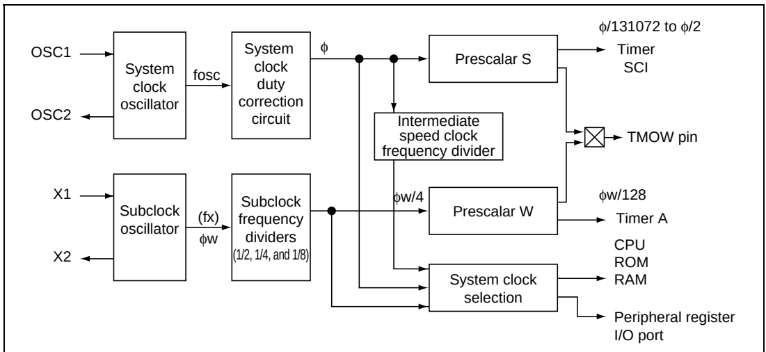
Figure 21.2 Clock Supply
