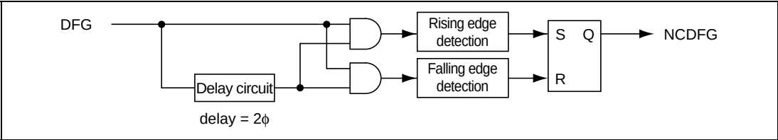
Figure 26.70 DFG Noise Removal Circuit
