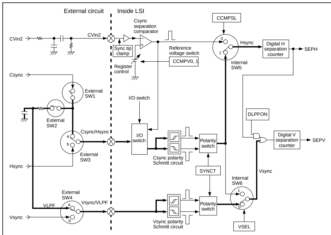
Figure 27.17 Sync Source Selection When Using the Csync Signal and the Vsync Schmitt Circuit
