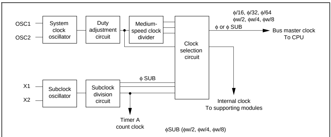
Figure 9.1 Block Diagram of Clock Pulse Generator
