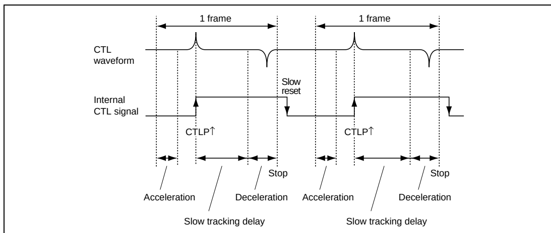
Figure 26.54 PB-CTL Waveform in Slow Mode Operation
