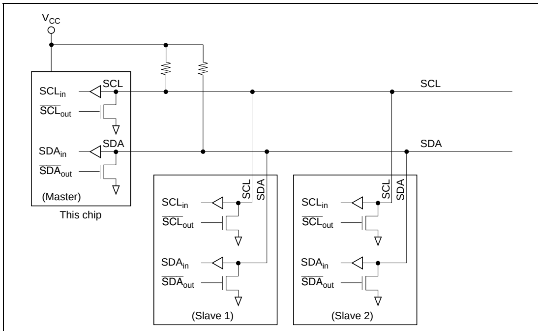
Figure 23.2 I²C Bus Interface Connections (Example: This Chip as Master)
