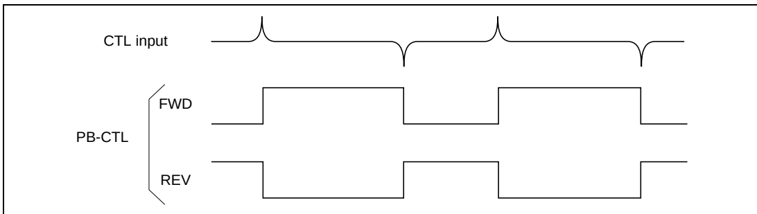
Figure 26.48 Internal PB-CTL Signal in Forward and Reverse
