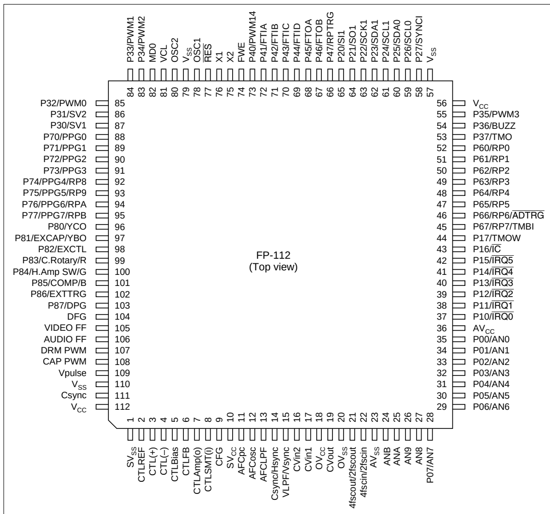
Figure 1.2 Pin Arrangement of H8S/2199 Series
