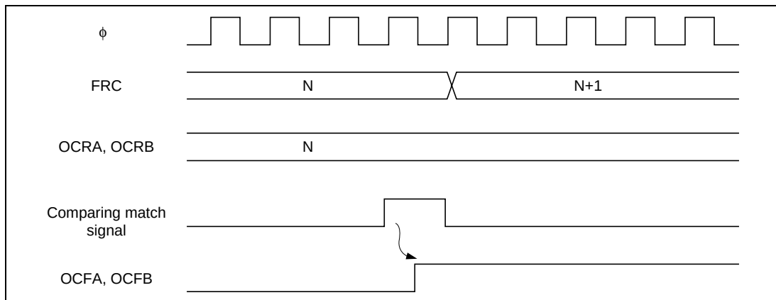
Figure 16.10 OCF Setting Up Timing
