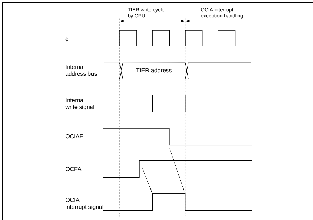
Figure 6.9 Contention between Interrupt Generation and Disabling
