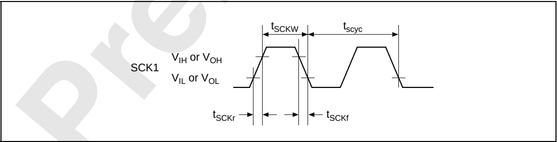
Figure 30.15 SCK1 Clock Timing
