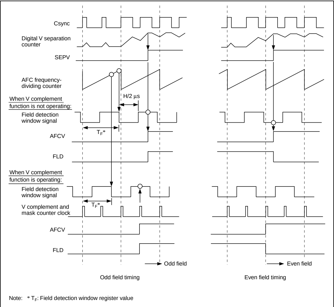
Figure 27.11 Field Detection Timing
