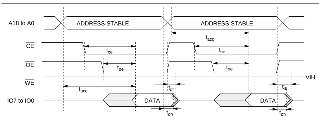
Figure 7.19 Timing Waveforms for \overline{\text{CE}}/\overline{\text{OE}} Clocked Read
