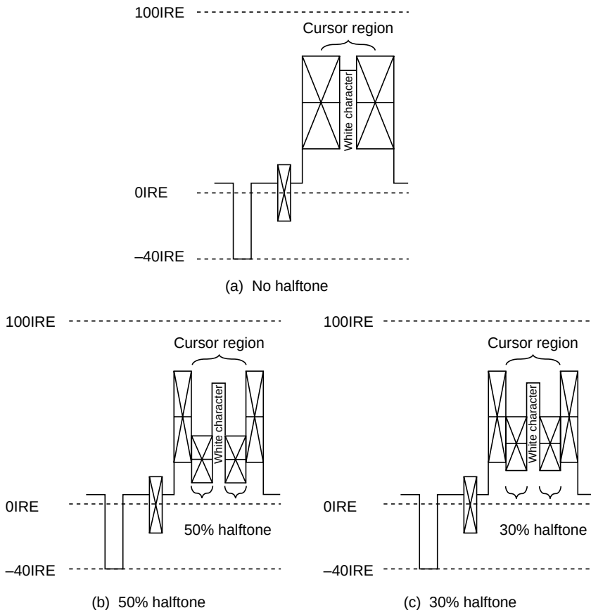
Figure 29.9 Halftone Level Examples (C.Video)
