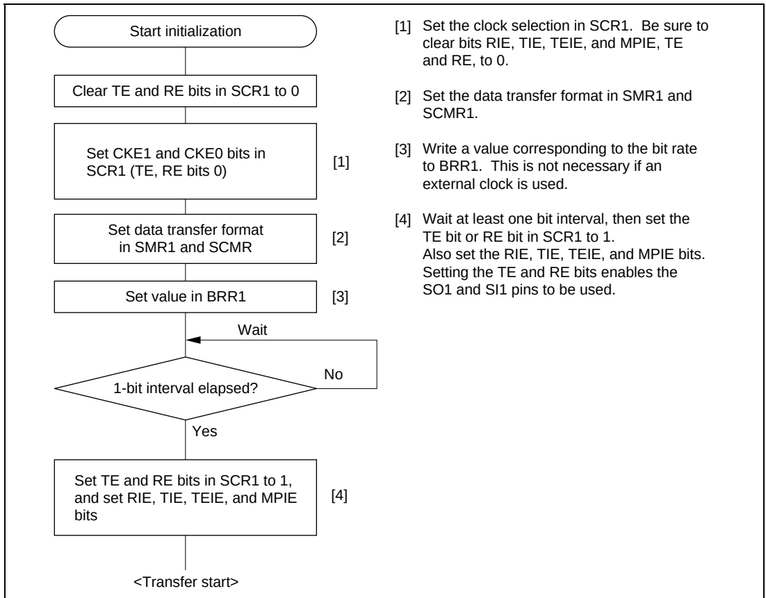
Figure 22.17 Sample SCI Initialization Flowchart
