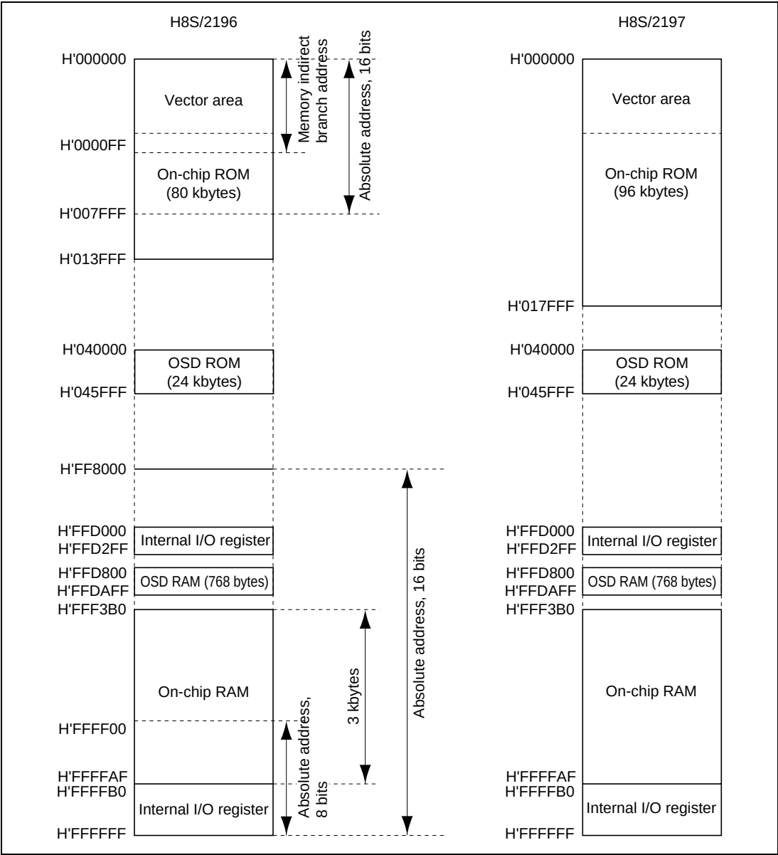
Figure 3.1 Address Map (1)
