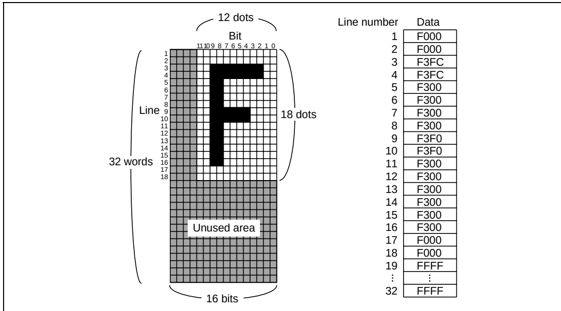
Figure 29.8 OSDROM Data Configuration (for the letter “F”)
