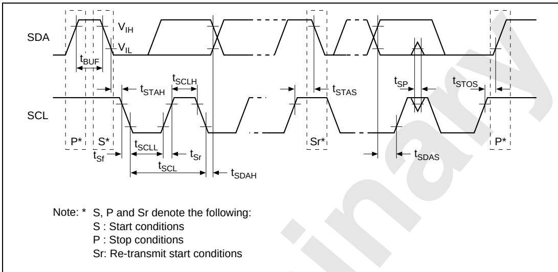
Figure 30.18 I²C Bus Interface I/O Timing
