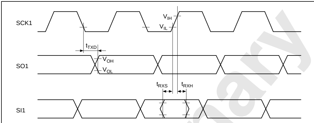
Figure 30.7 SCI I/O Timing/Clock Synchronization Mode
