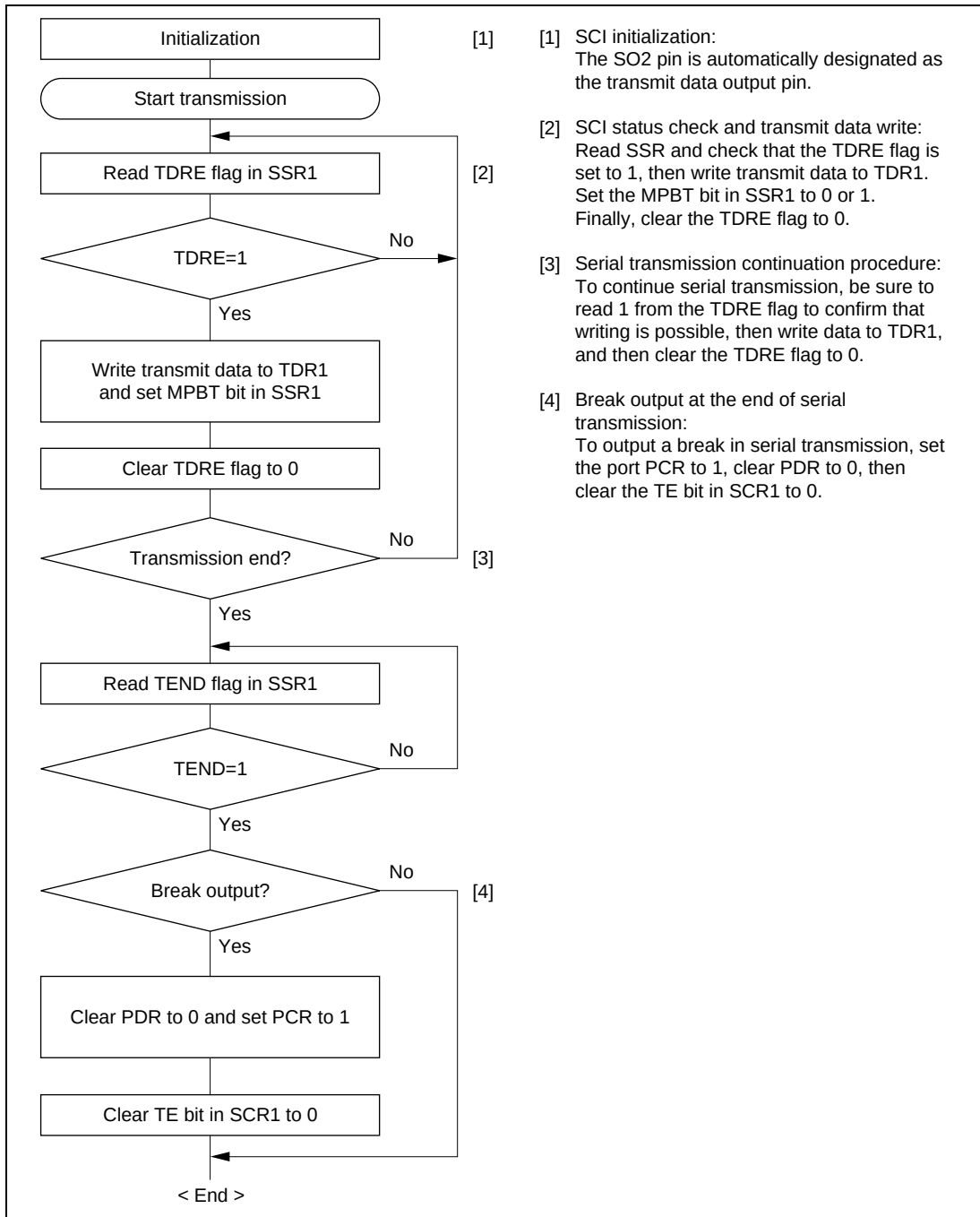
Figure 22.11 Sample Multiprocessor Serial Transmission Flowchart
