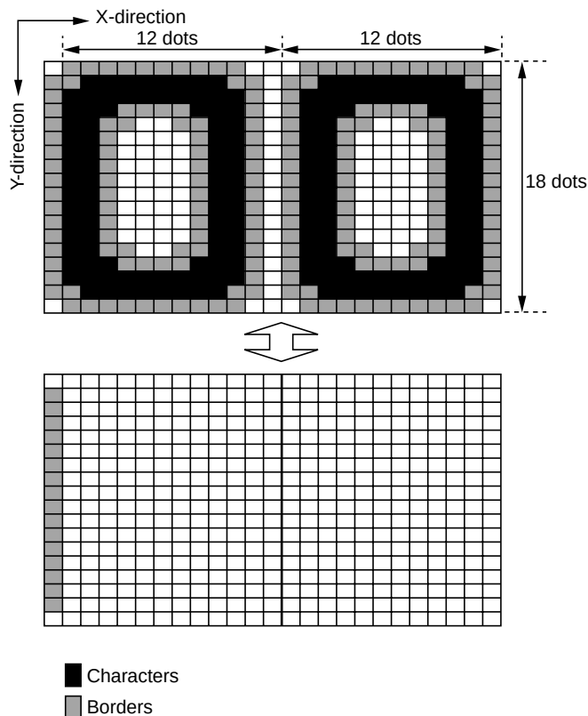
Figure 29.19 Example of Blinking with Borders Extending beyond the Display Frame
