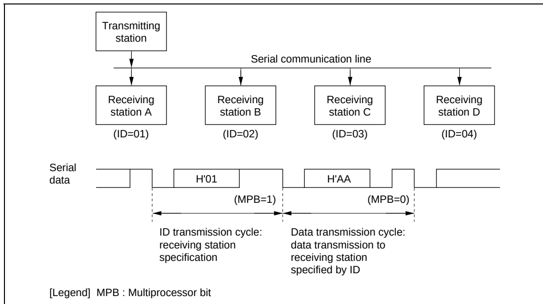
Figure 22.10 Example of Inter-Processor Communication Using Multiprocessor Format (Transmission of Data H'AA to Receiving Station A)
