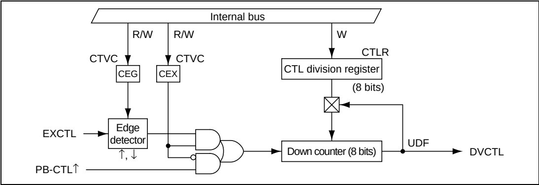
Figure 26.63 CTL Frequency Divider
