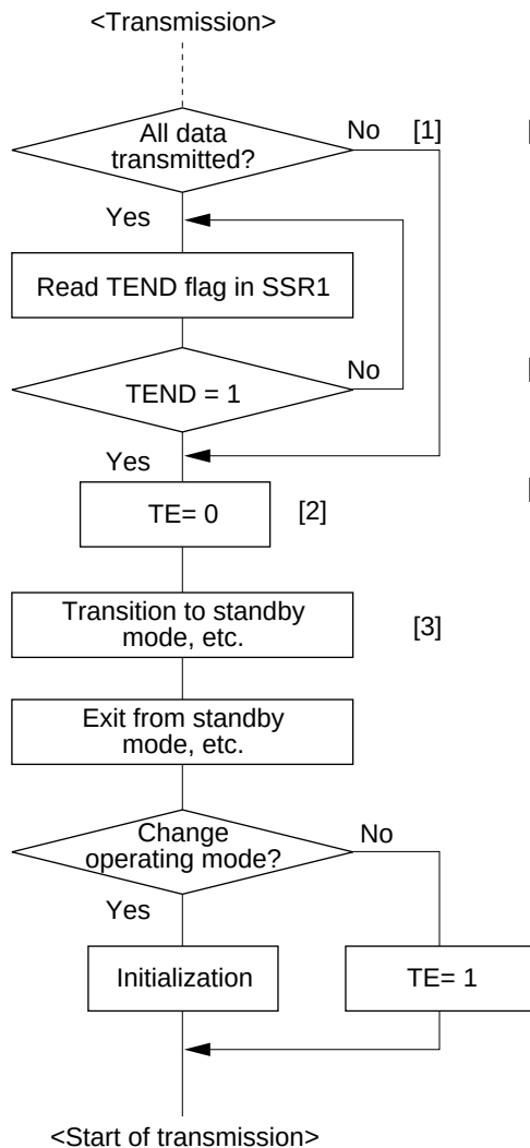
Figure 22.24 Sample Flowchart for Mode Transition during Transmission
