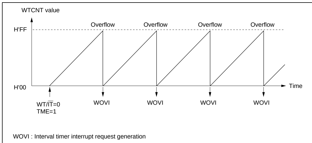
Figure 17.4 Operation in Interval Timer Mode
