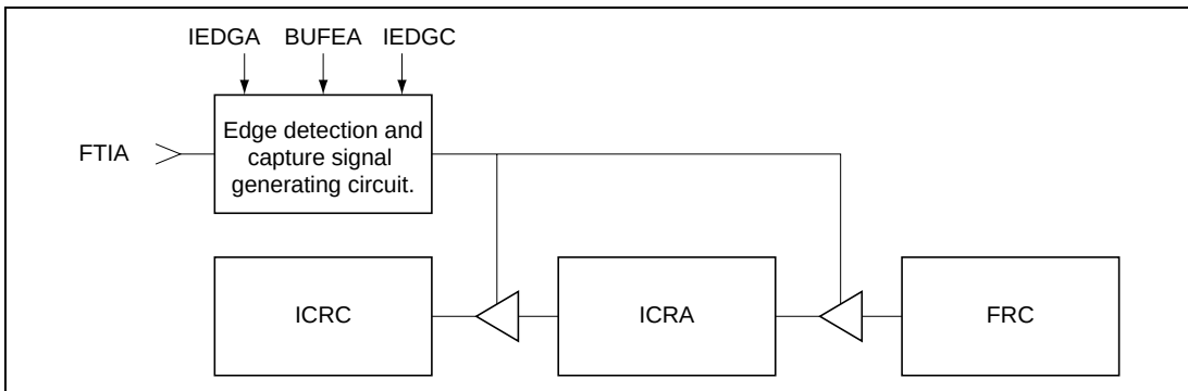
Figure 16.2 Buffer Operation (Example)
