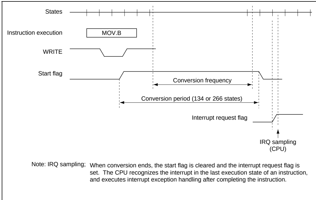
Figure 24.2 Internal Operation of A/D Converter
