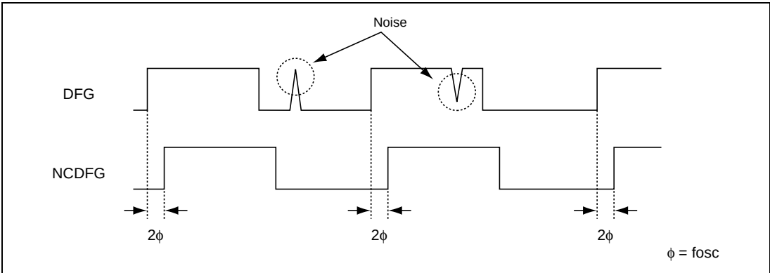
Figure 26.71 NCDFG Signal
