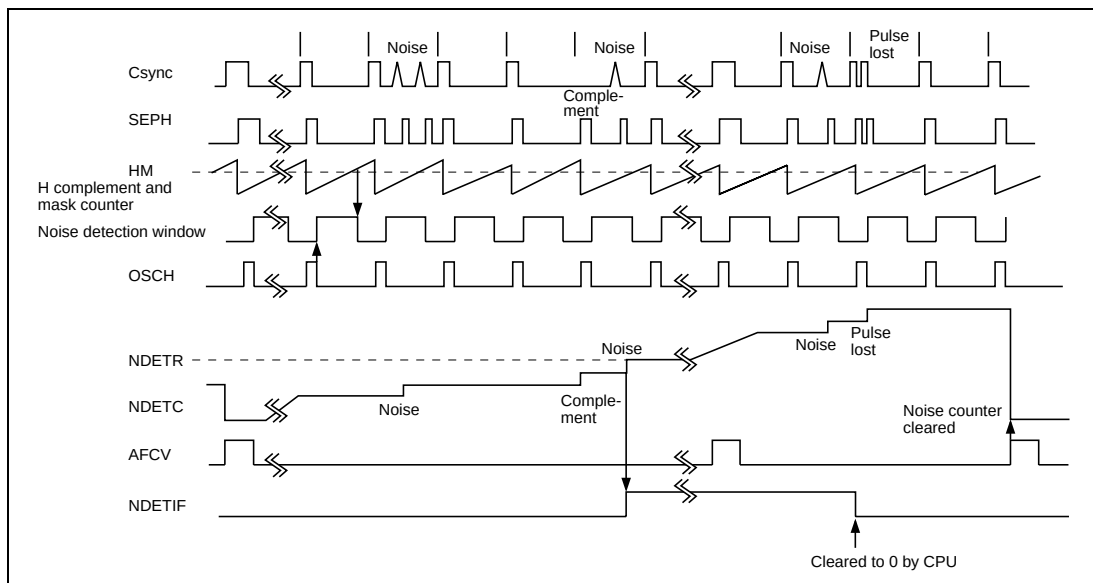
Figure 27.13 Noise Detection Window Setting and Noise Counting Timing
