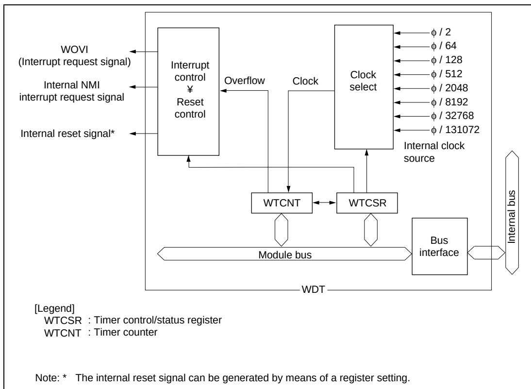
Figure 17.1 Block Diagram of WDT
