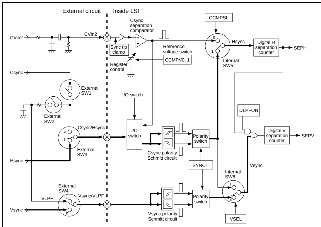
Figure 27.19 Sync Source Selection When Using the Hsync and Vsync Signals Separately
