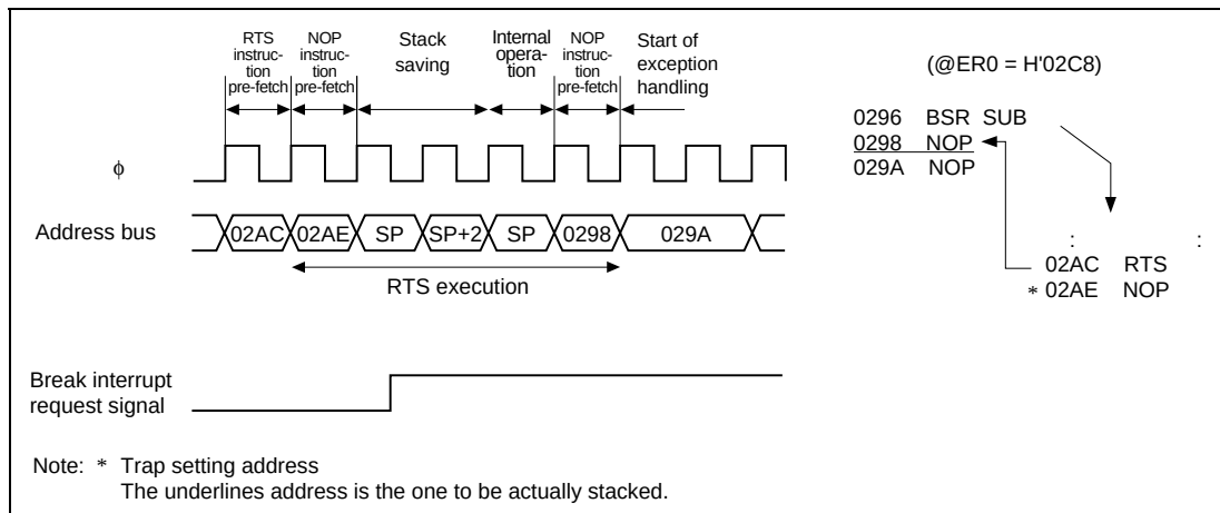
Figure 25.15 RTS Instruction
