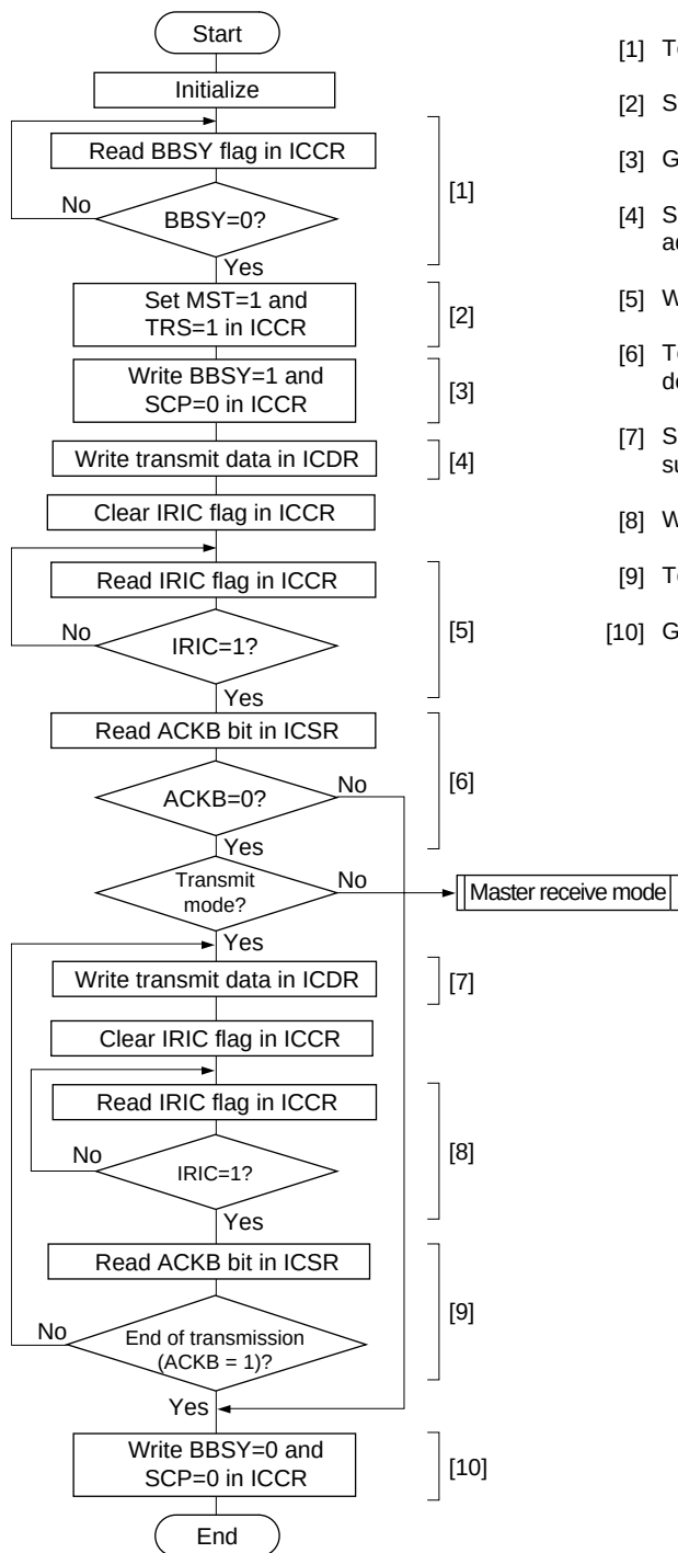
Figure 23.14 Flowchart for Master Transmit Mode (Example)
