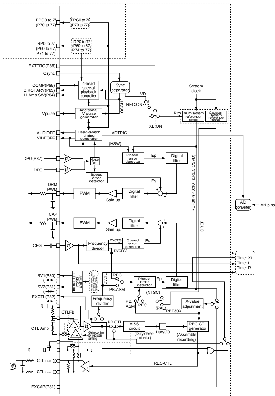
Figure 26.1 Block Diagram of Servo Circuits
