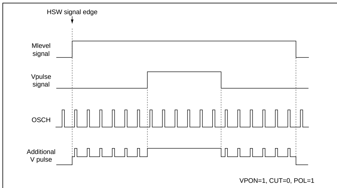
Figure 26.45 Additional V Pulse when Positive Polarity Is Specified
