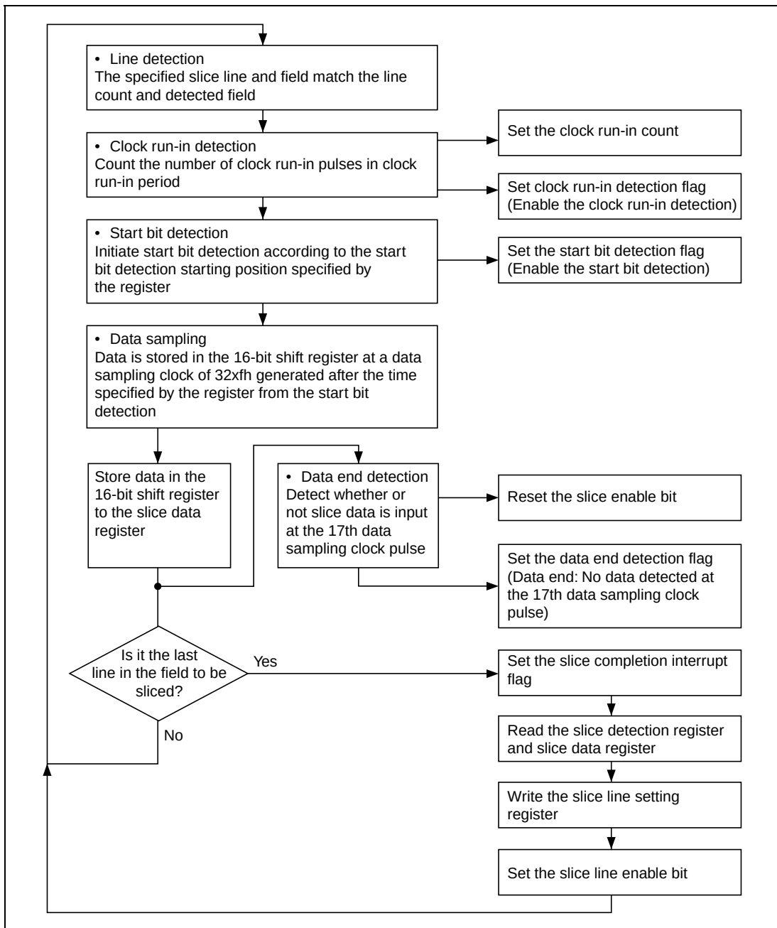
Figure 28.11 Slice Sequence
