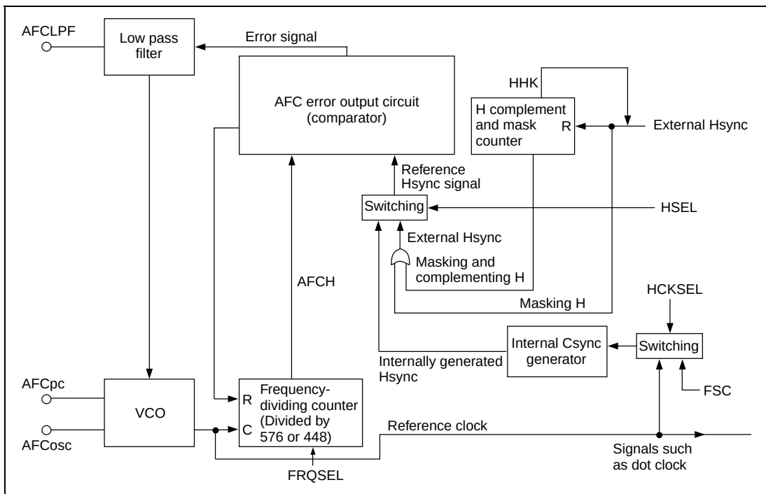
Figure 27.20 AFC Configuration
