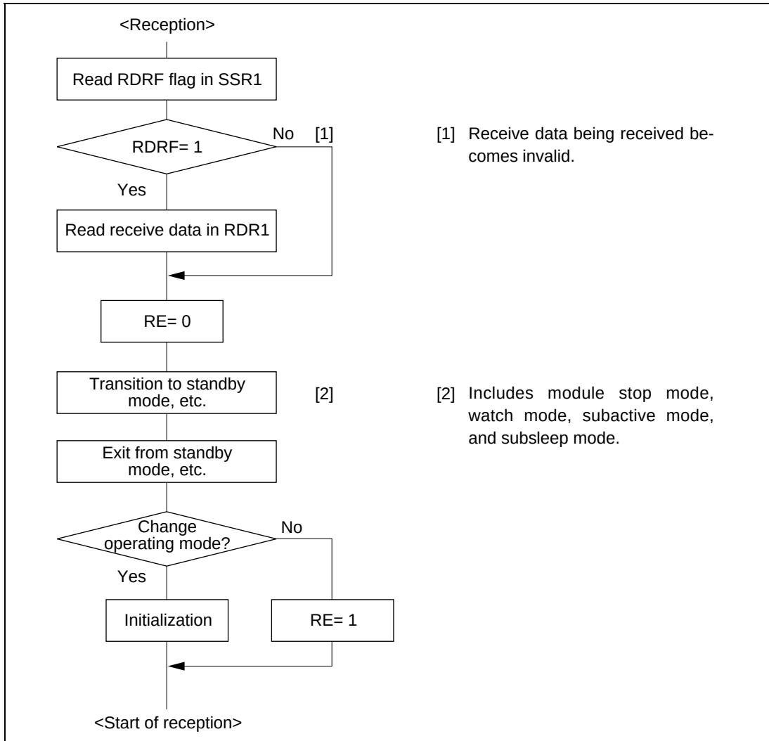
Figure 22.27 Sample Flowchart for Mode Transition during Reception
