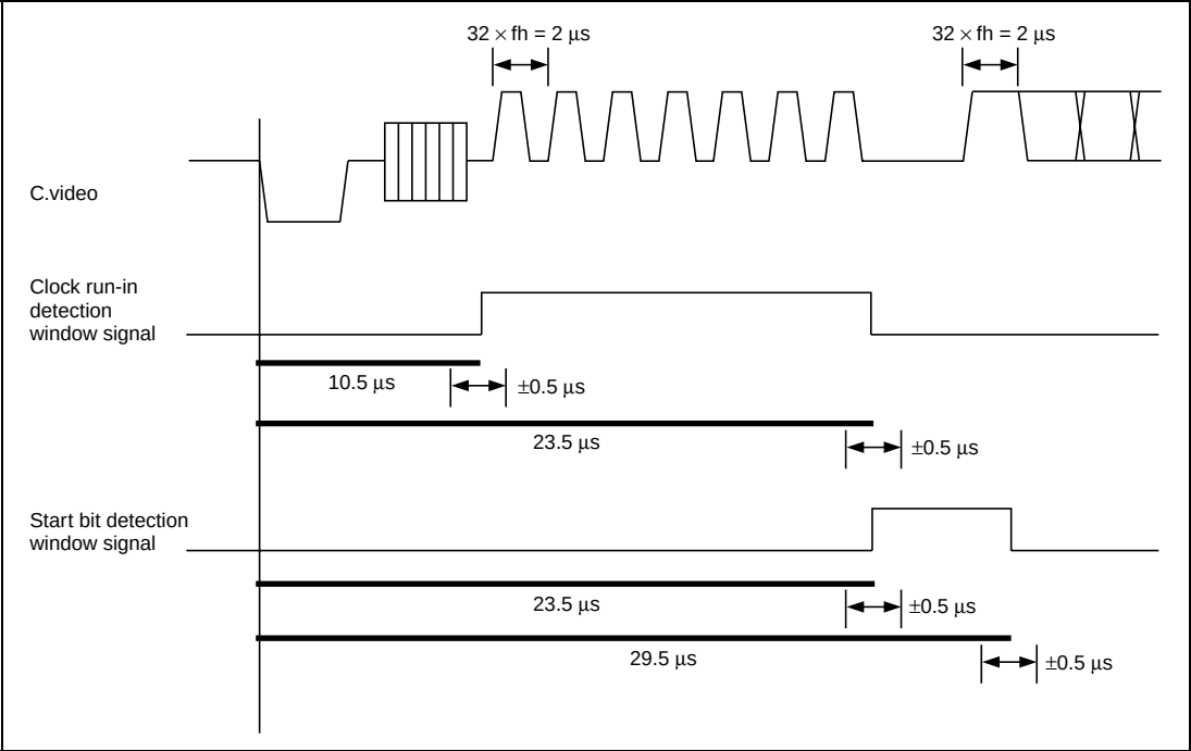
Figure 27.14 Timing for Generating Clock Run-in Detection Window Signal and Start Bit Detection Window Signal
