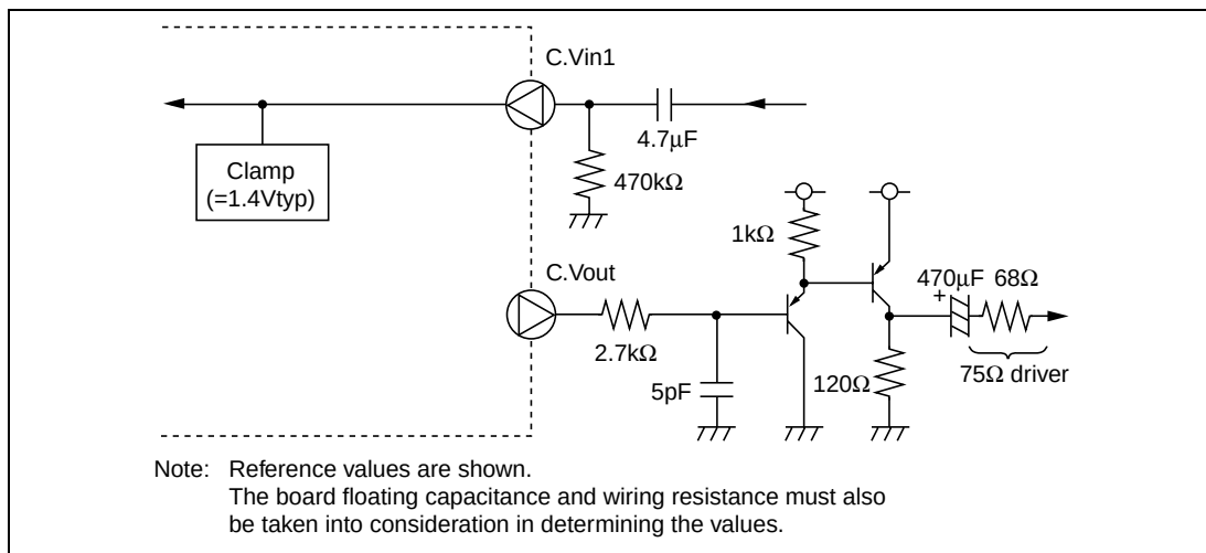
Figure E.5 Example of External Circuit for OSD
