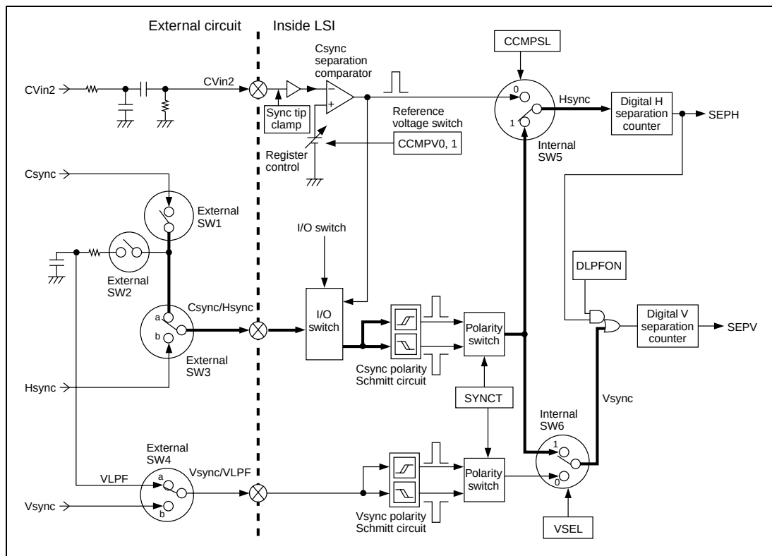
Figure 27.18 Sync Source Selection When Using the Csync Signal and the Csync Schmitt Circuit
