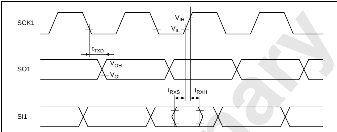
Figure 30.16 SCI I/O Timing/Clock Synchronization Mode
