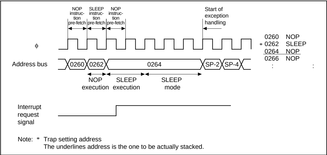
Figure 25.17 SLEEP Instruction (2)
