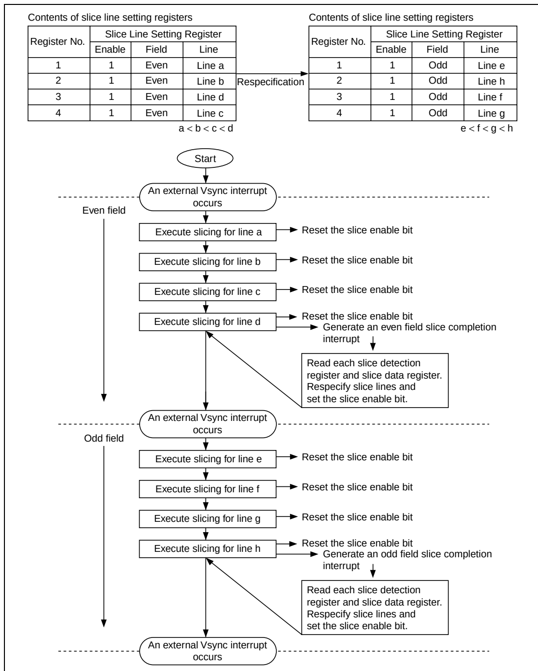
Figure 28.10 Example of Slice Line Specification and Operation (2)
