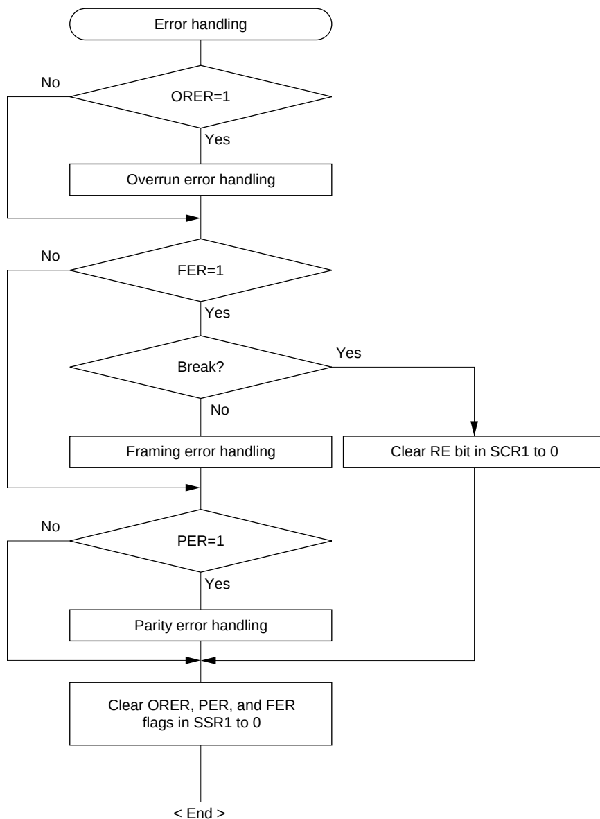
Figure 22.8 Sample Serial Reception Data Flowchart (2)
