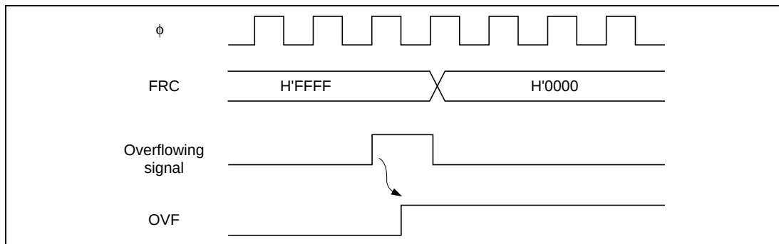
Figure 16.11 OVF Setting Up Timing
