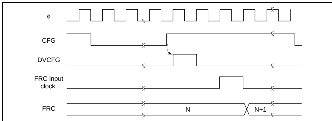
Figure 16.4 Count Timing for CFG Clock Operation
