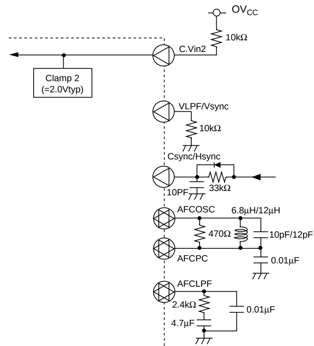
Figure E.7 Example of External Circuit for Sync Separator and Data Slicer (2) Separation from Csync)
