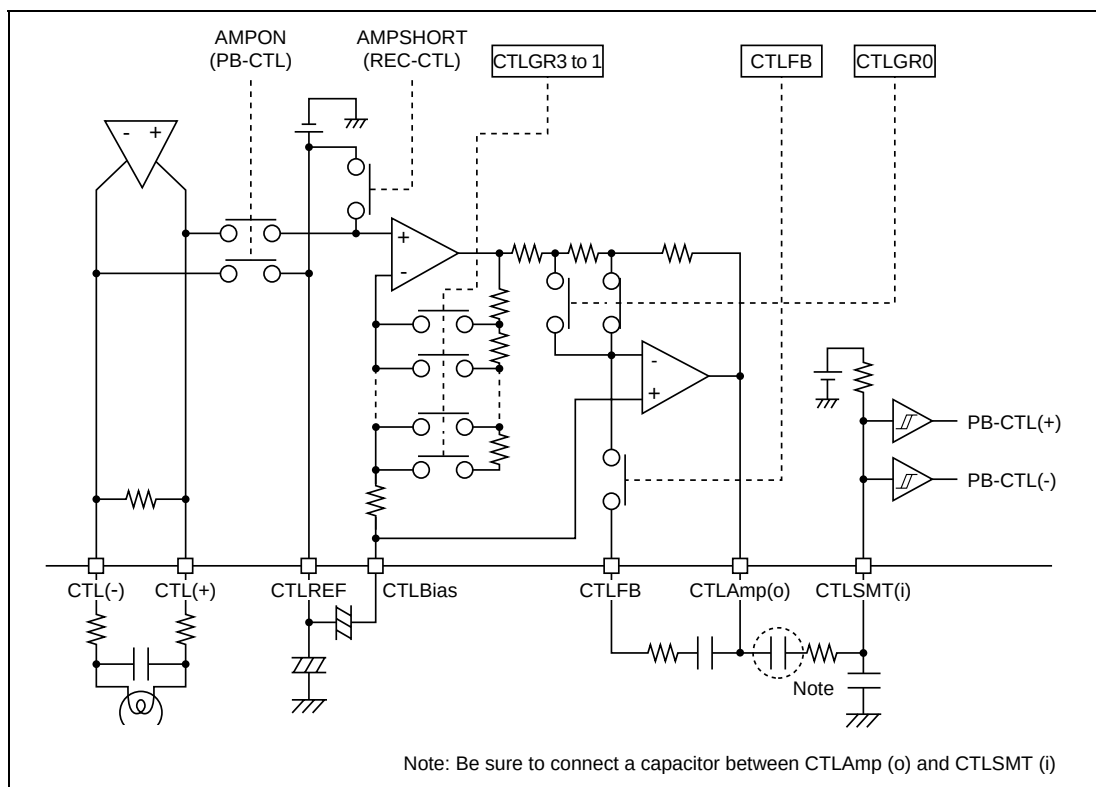
Figure 26.4 CTL Input Circuit
