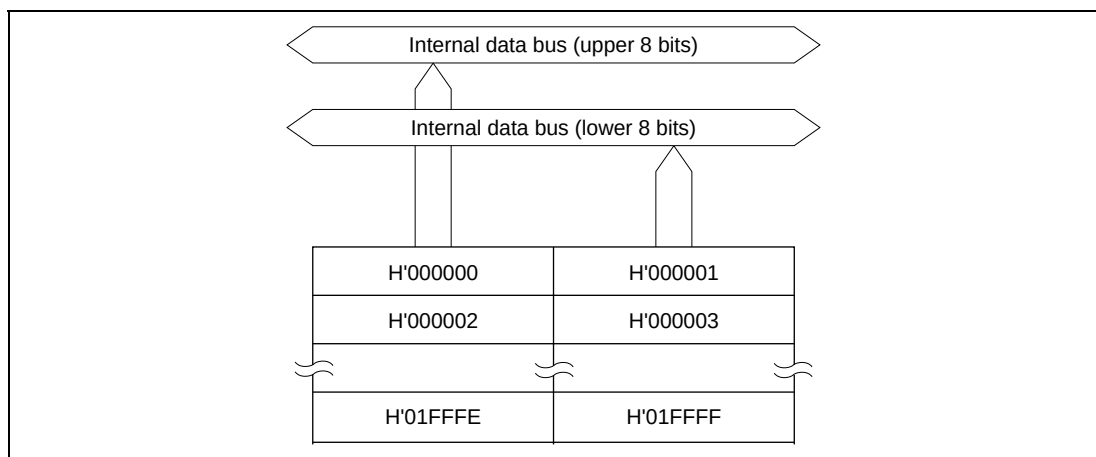
Figure 7.1 ROM Block Diagram (H8S/2199)
