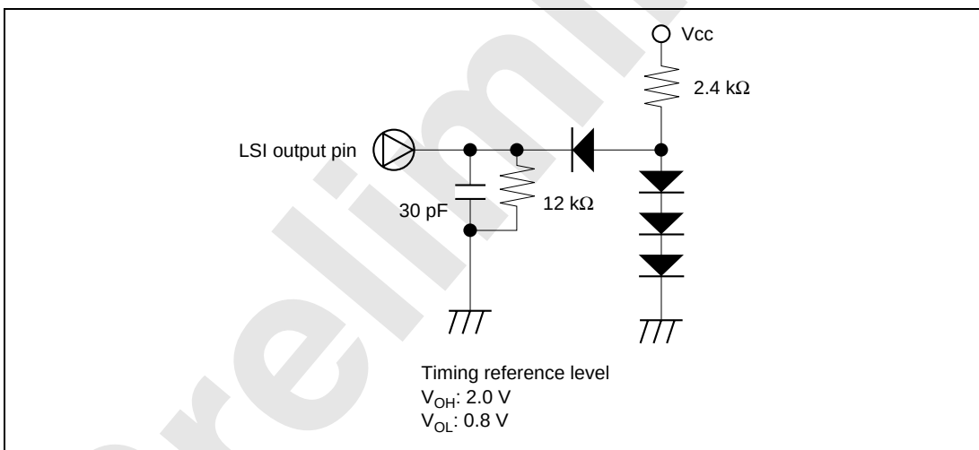
Figure 30.8 Output Load Conditions
