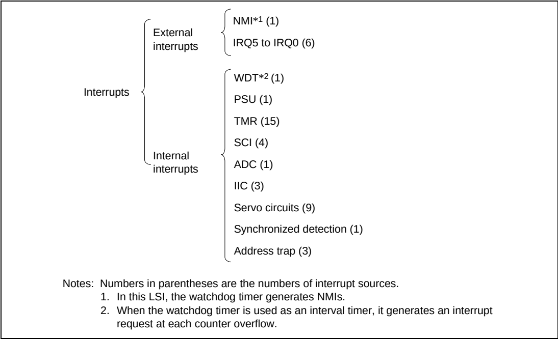
Figure 5.3 Interrupt Sources and Number of Interrupts
