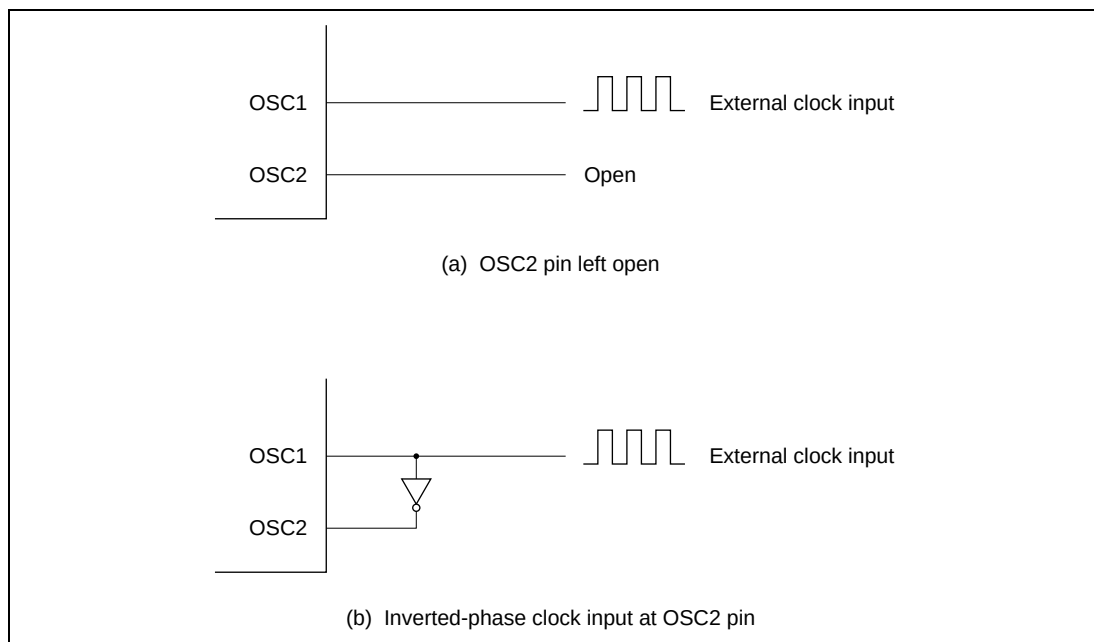
Figure 9.5 External Clock Input (Examples)
