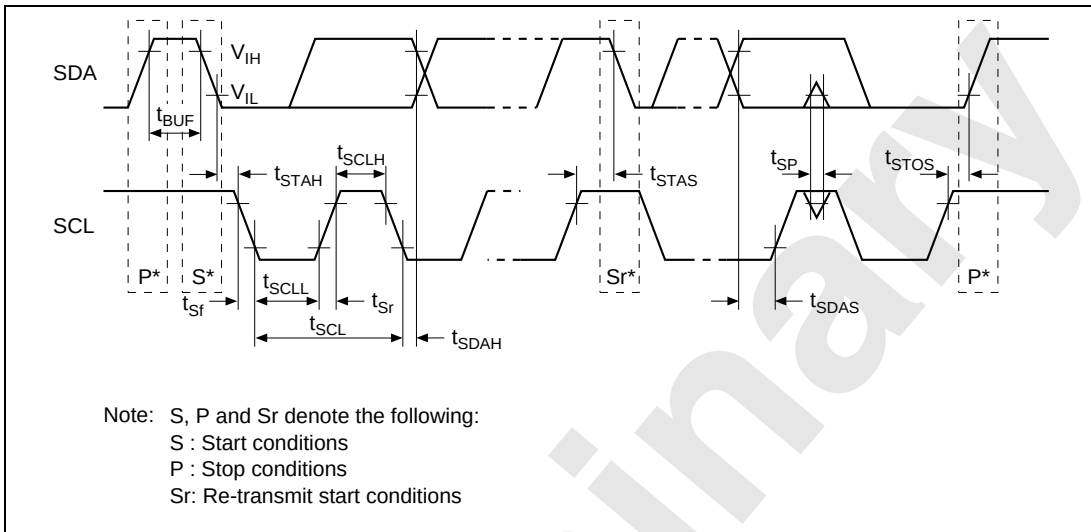
Figure 30.9 I²C Bus Interface I/O Timing
