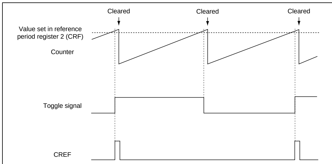
Figure 26.13 Generation of CREF Signal
