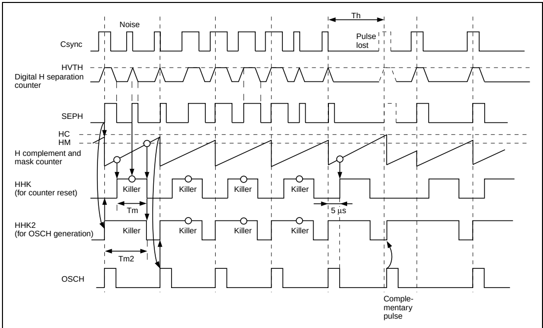
Figure 27.12 Complement and Mask Timing of the H Complement and Mask Counter
