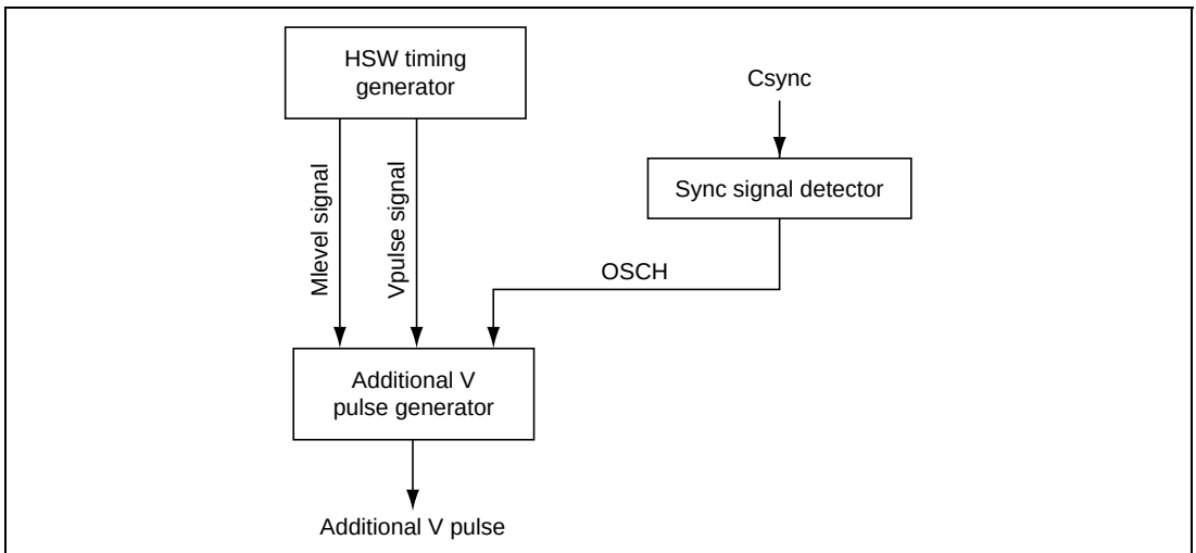
Figure 26.43 Additional V Pulse Control Circuit
