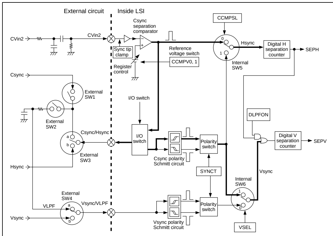
Figure 27.16 Sync Source Selection When Using the CVin2 Signal and the Csync Schmitt Circuit
