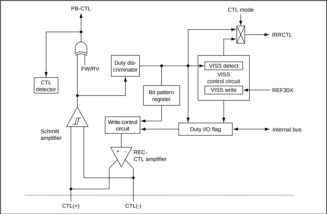
Figure 26.47 Block Diagram of CTL Circuit
