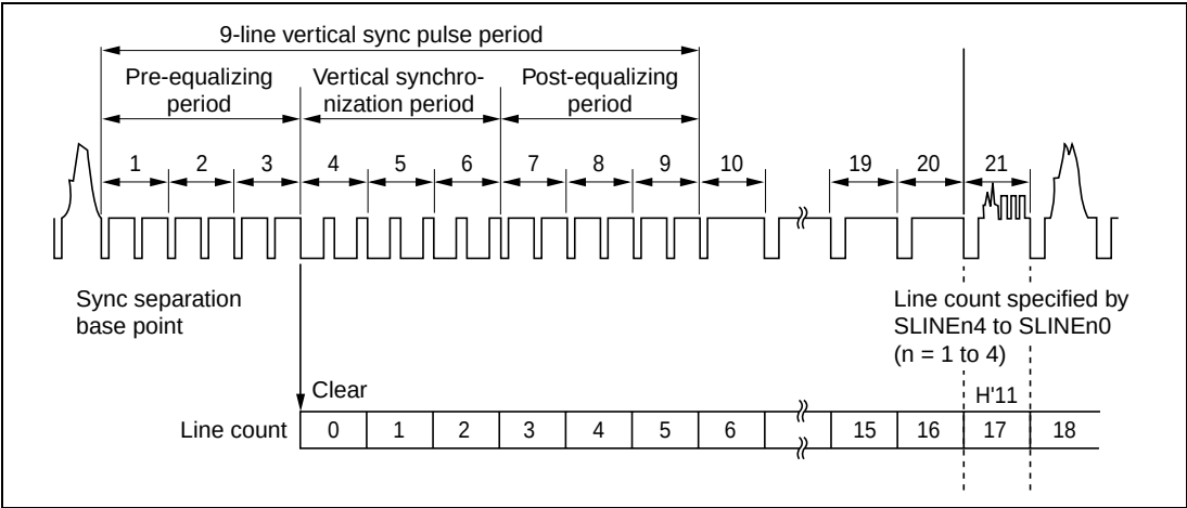
Figure 28.4 Line Count
