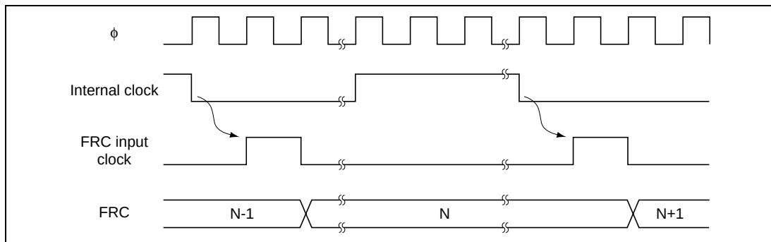
Figure 16.3 Count Timing for Internal Clock Operation
