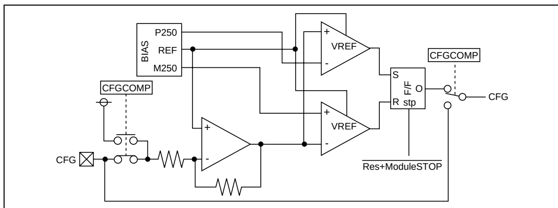
Figure 26.3 CFG Input Circuit
