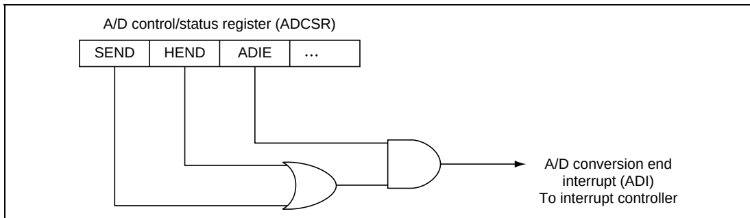
Figure 24.4 Block Diagram of A/D Conversion End Interrupt
