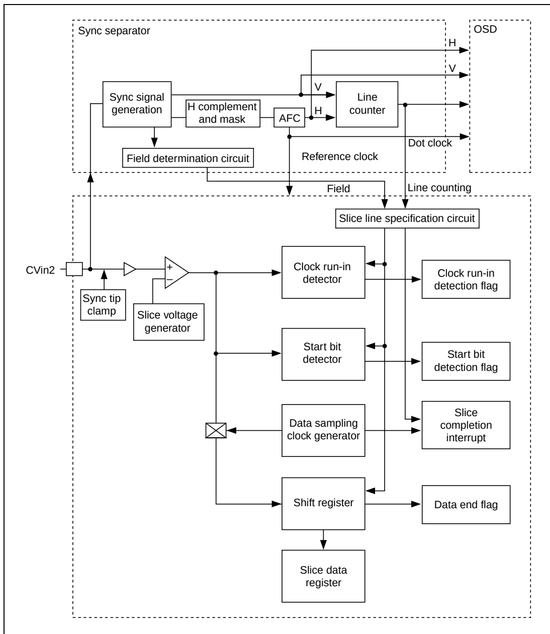
Figure 28.1 Data Slicer Block Diagram
