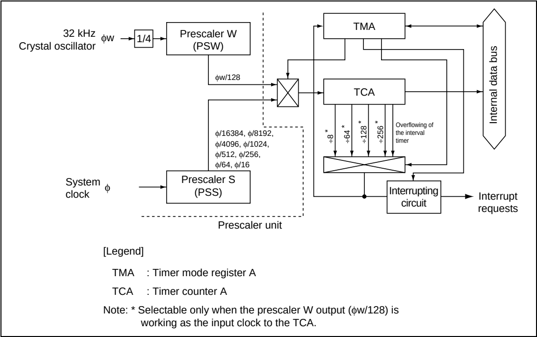
Figure 11.1 Block Diagram of Timer A
