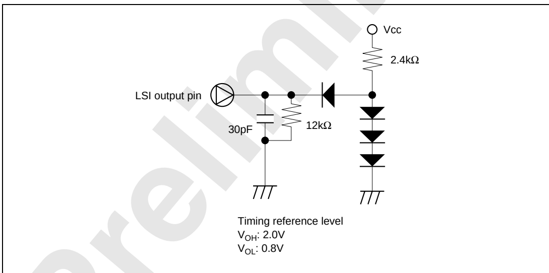
Figure 30.17 Output Load Conditions
