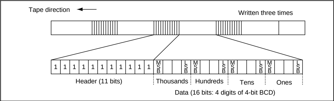
Figure 26.58 VASS (Index) Format
