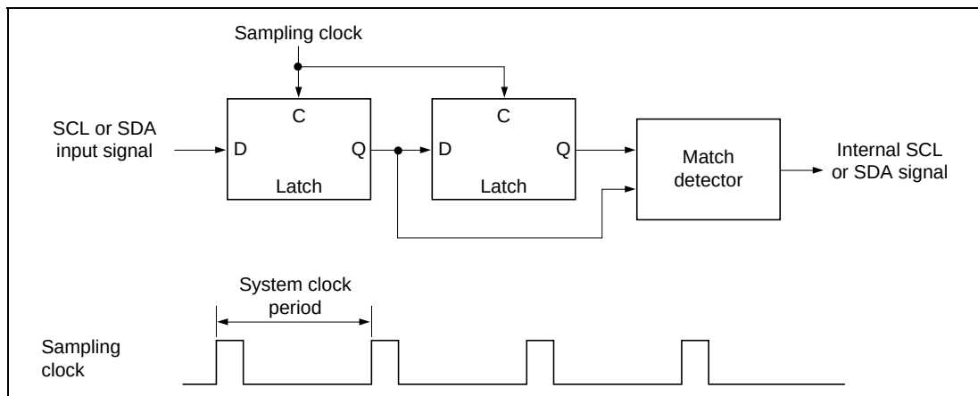
Figure 23.13 Block Diagram of Noise Canceler
