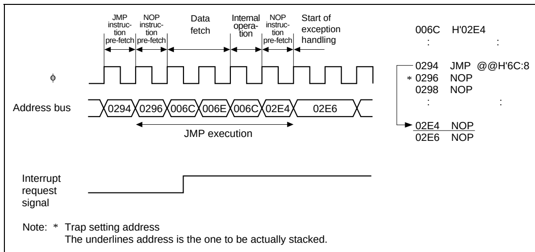
Figure 25.14 JMP Instruction (Memory Indirect)
