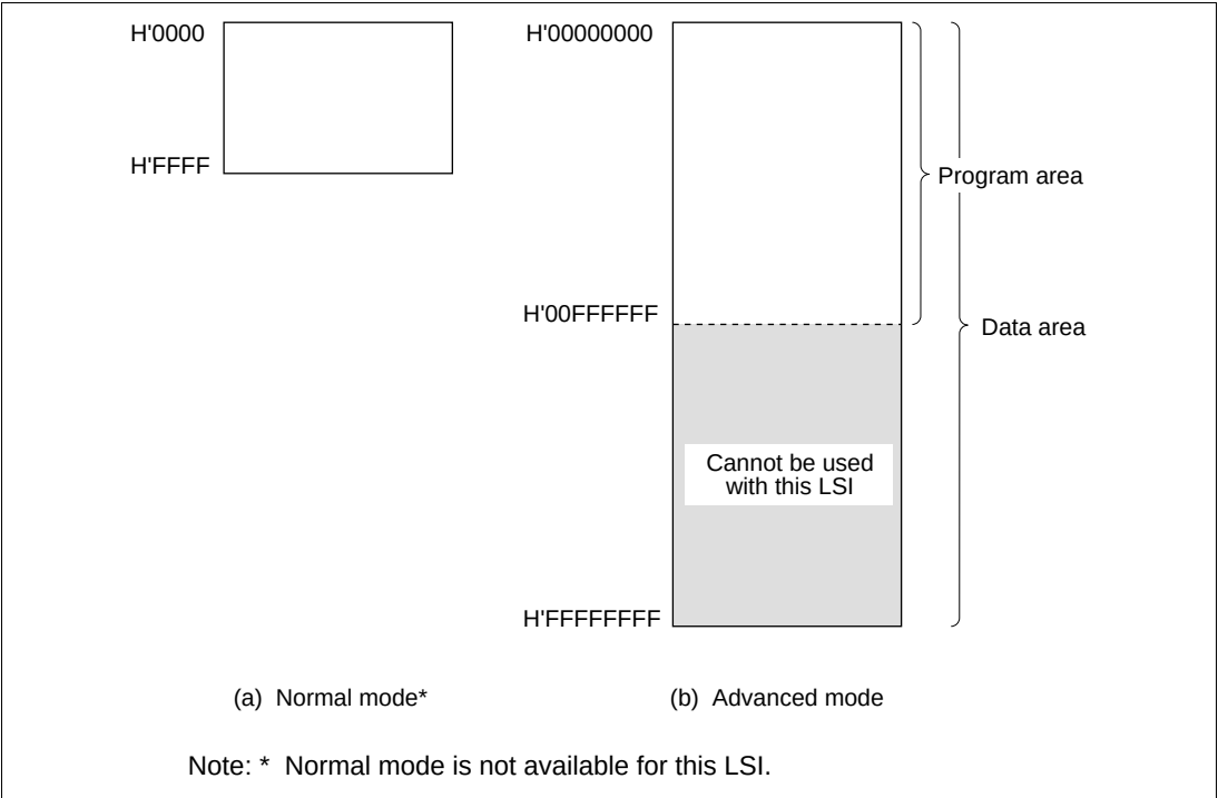
Figure 2.6 Memory Map
