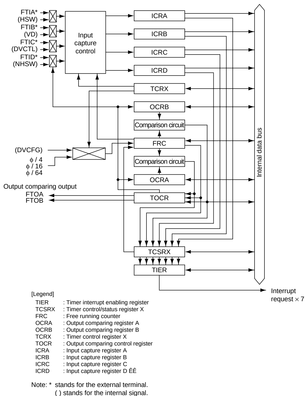
Figure 16.1 Block Diagram of Timer X1
