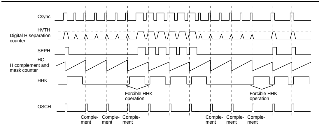
Figure 27.7 Timing of HHK Operation
