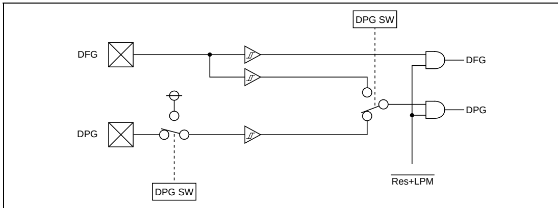
Figure 26.2 Input Circuit of DFG and DPG
