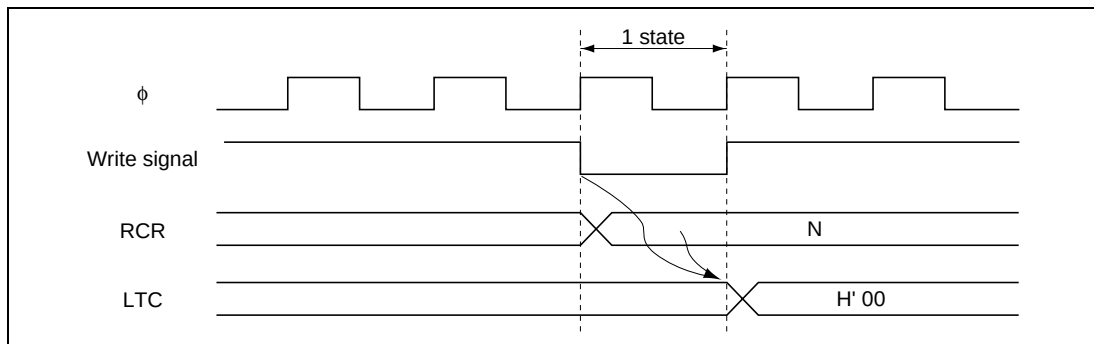
Figure 14.2 RCR Writing and LTC Clearing Timing Chart
