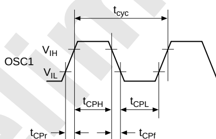
Figure 30.10 System Clock Timing
