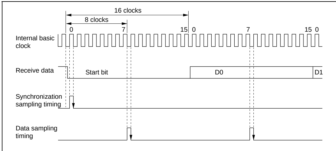
Figure 22.23 Receive Data Sampling Timing in Asynchronous Mode
