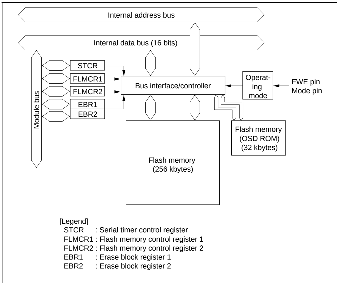
Figure 7.2 Block Diagram of Flash Memory (H8S/2199 Only)
