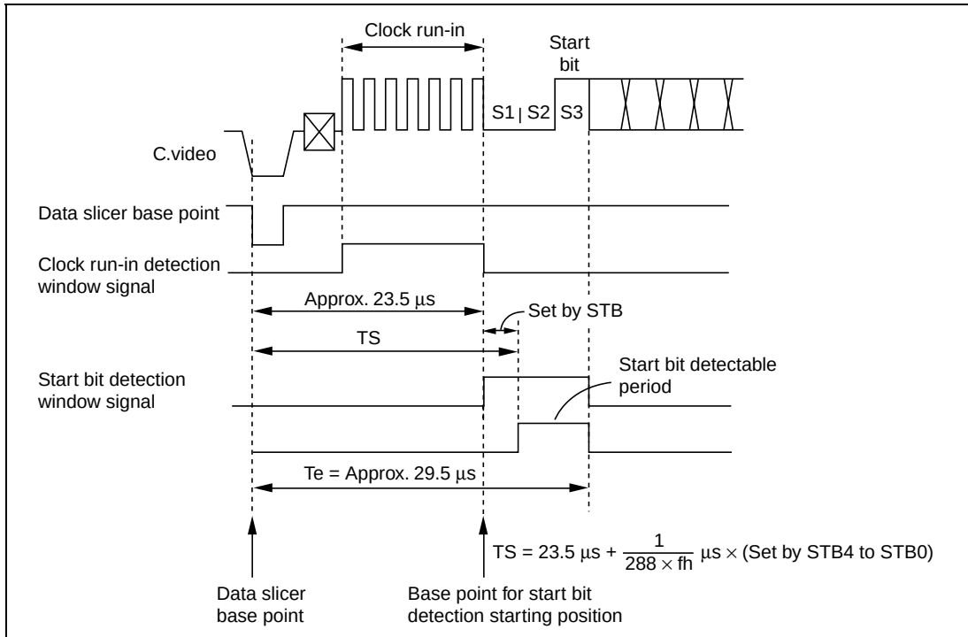
Figure 28.2 Data Slicer Base Point and Start Bit Detection Starting Position
