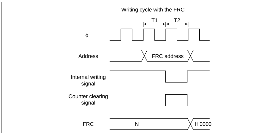
Figure 16.13 Competition between Writing and Clearing with the FRC
