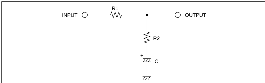
Figure 26.40 Lag-Lead Filter
