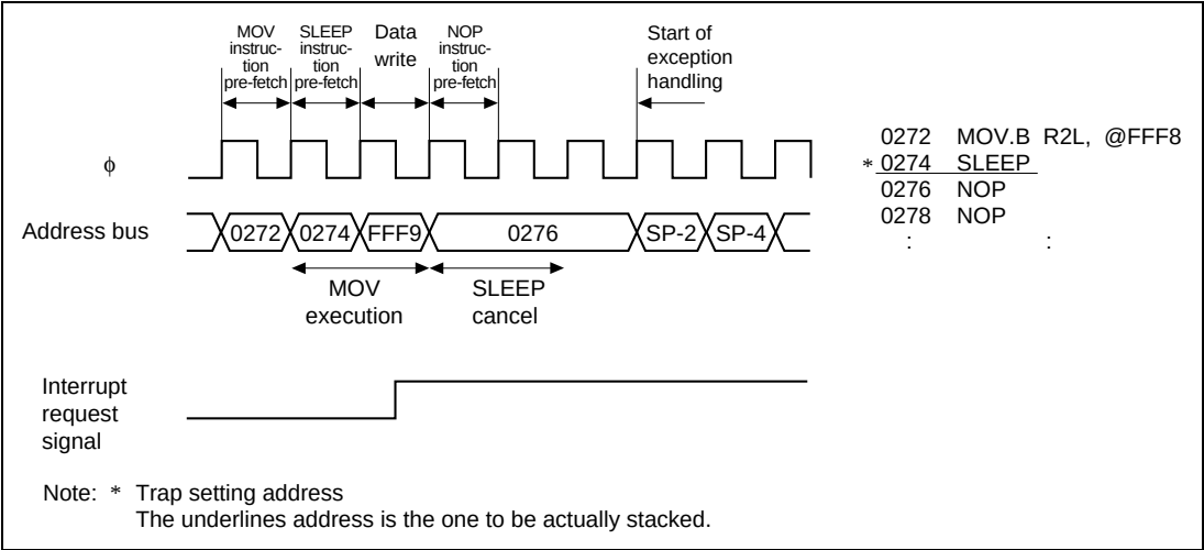
Figure 25.16 SLEEP Instruction (1)
