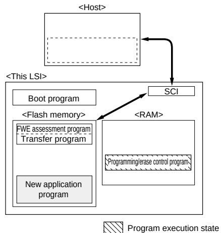
Figure 7.5 User Program Mode (Example)
