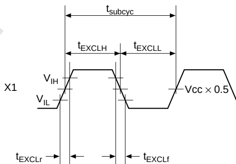
Figure 30.2 Subclock Input Timing
