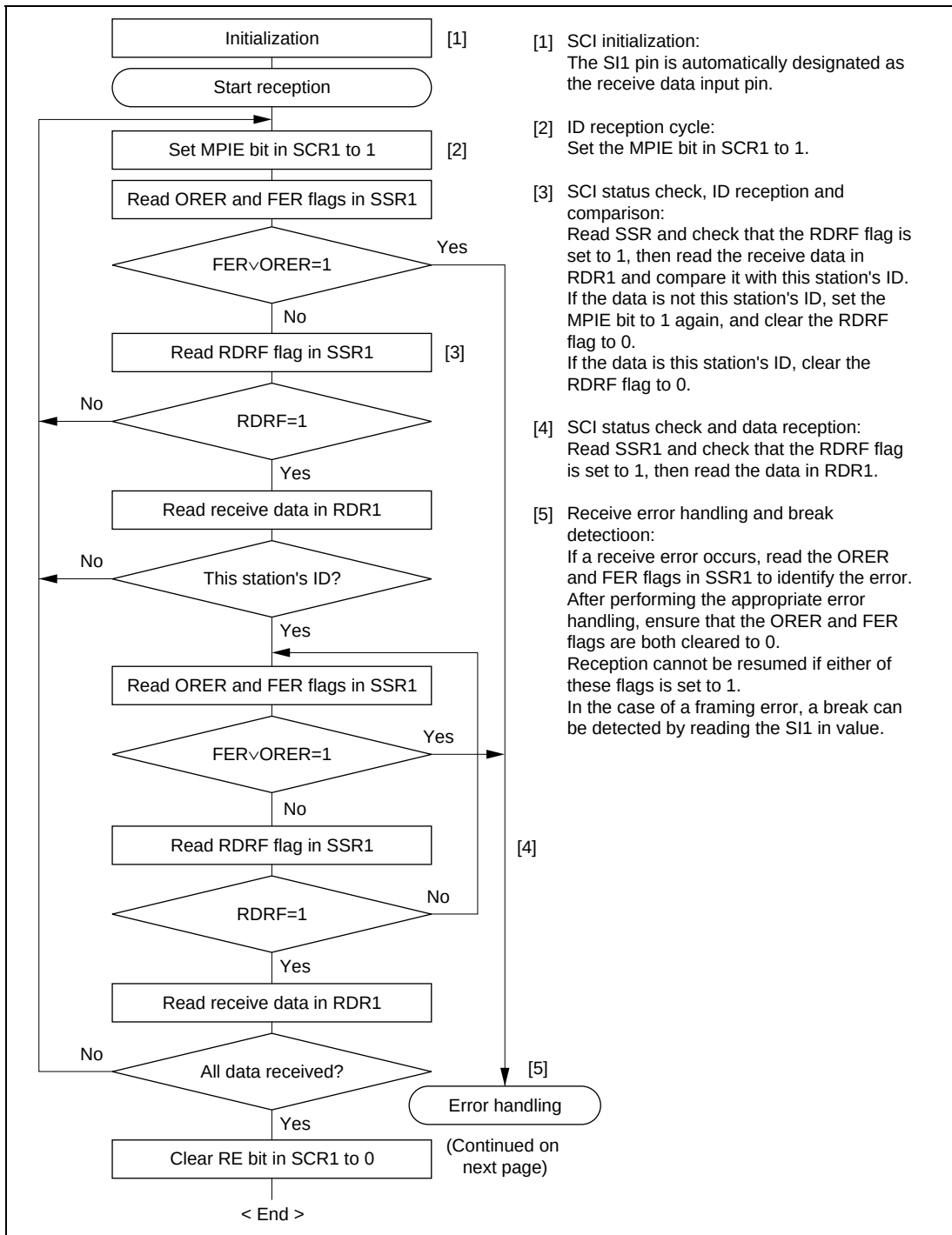
Figure 22.13 Sample Multiprocessor Serial Reception Flowchart (1)
