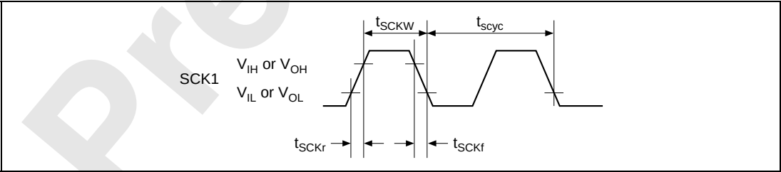
Figure 30.6 SCK1 Clock Timing
