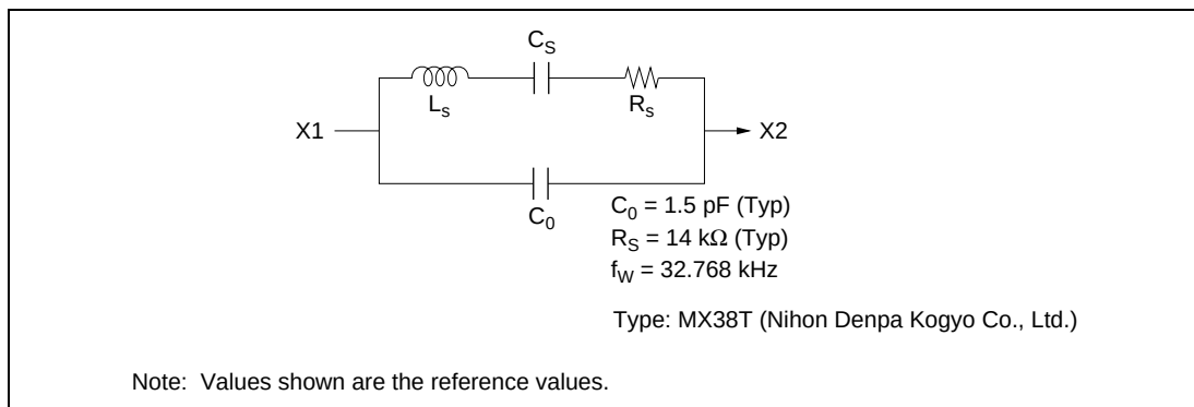
Figure 9.9 32.768 kHz Crystal Resonator Equivalent Circuit
