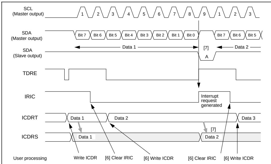
Figure 23.7 Example of Continuous Transmission Timing in Master Transmit Mode (MLS = WAIT = 0)
