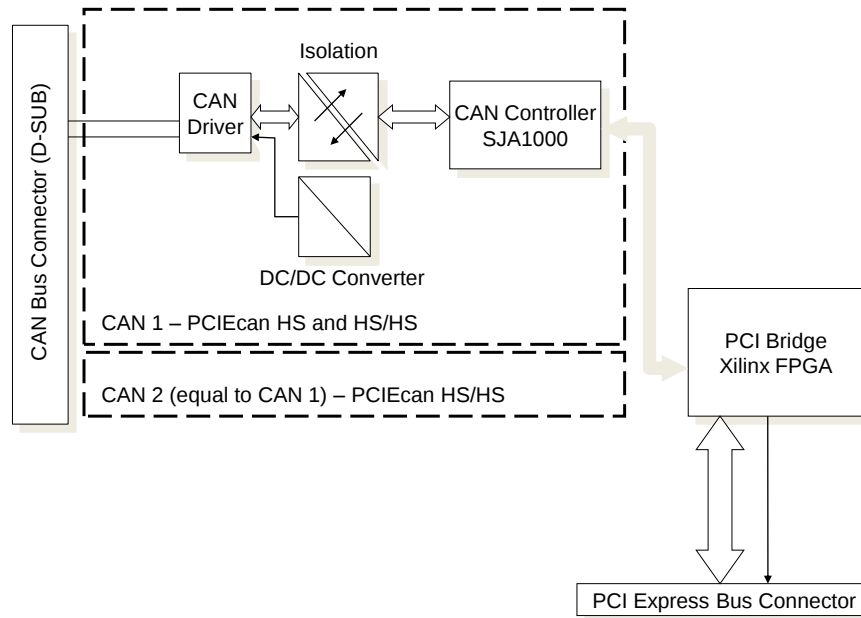
Figure 1 Block diagram for Kvaser PCIEcan HS/HS.
