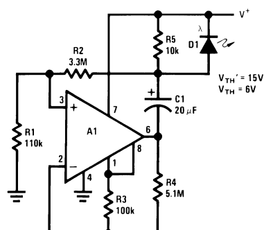
Figure 62. Battery-threshold Indicator
