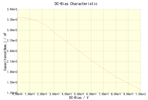
C3225X7R2A334M200AA
