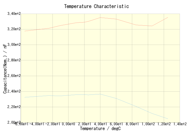
C3225X7R2A334M200AA(DC Bias = 0V) C3225X7R2A334M200AA(DC Bias = 50V)
