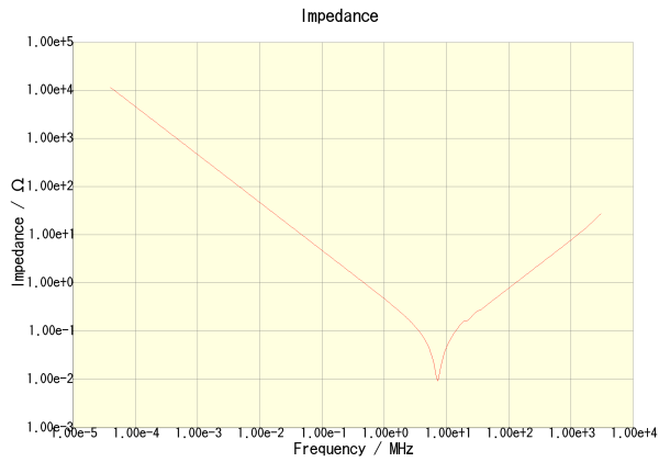
C3225X7R2A334M200AA
