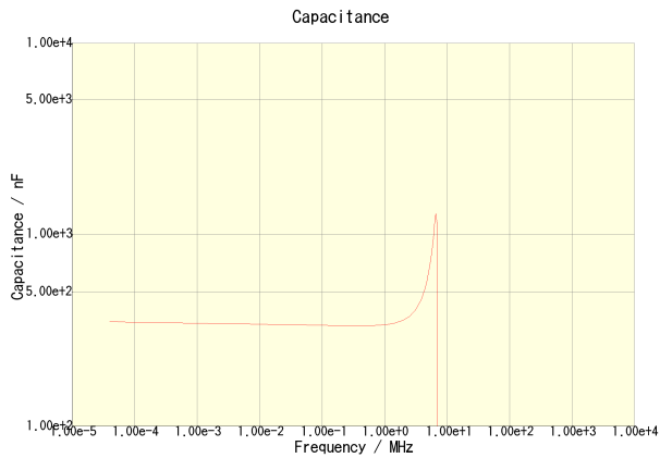
C3225X7R2A334M200AA
