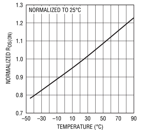
R_{DS(ON)} Change vs Temperature
