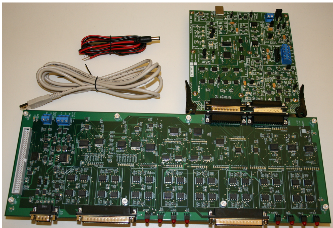
Figure 1. Hardware Included with the Multi-Cal-System EVM Kit
