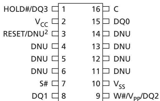
Figure 3: 16-Lead, Plastic Small Outline – S016 (Top View)
