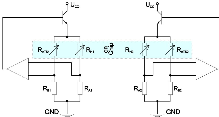
Figure 3: Above is shown an example of a measurement electronics using a Wheatstone-bridge. The resistors R_{Ax} and R_{Bx} need to be trimmed to operate the heater at a defined over-temperature
