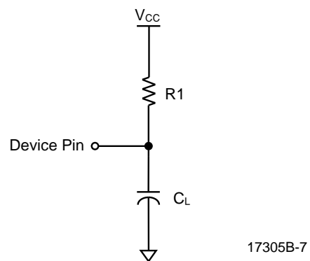
B. Open-Drain Outputs ( \overline{\text{RDY}} , \overline{\text{INT}} )
