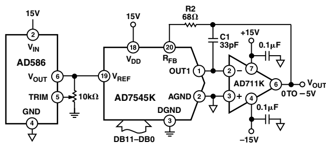
Figure 11. Low-Power 12-Bit CMOS DAC Application
