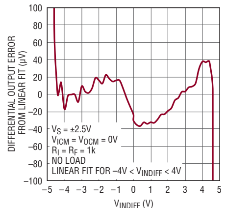
DC Linearity
