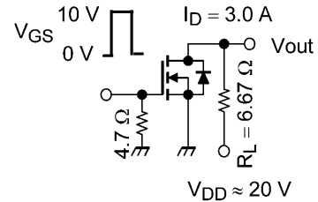
Fig. 6.2.2 Switching Time Test Circuit (N-ch)
