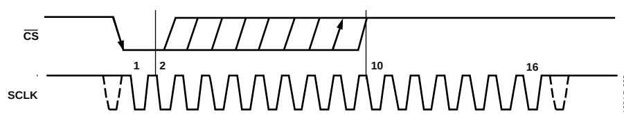
Figure 20. Entering Partial Power-Down Mode
