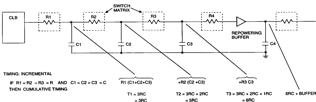
Figure 28. Interconnection Timing Example. Use of the XACT timing calculator
