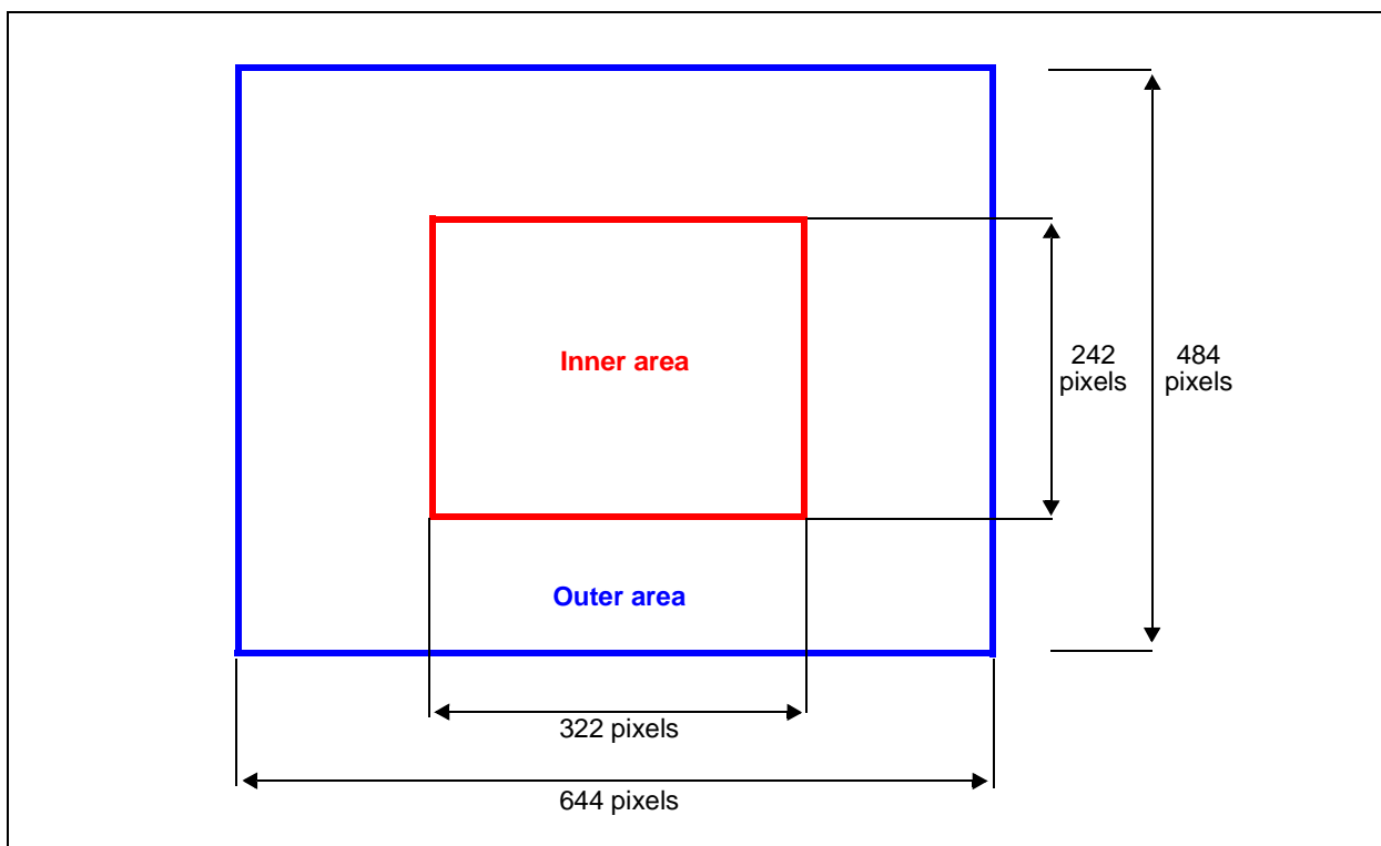
Figure 30: VV6501 array
