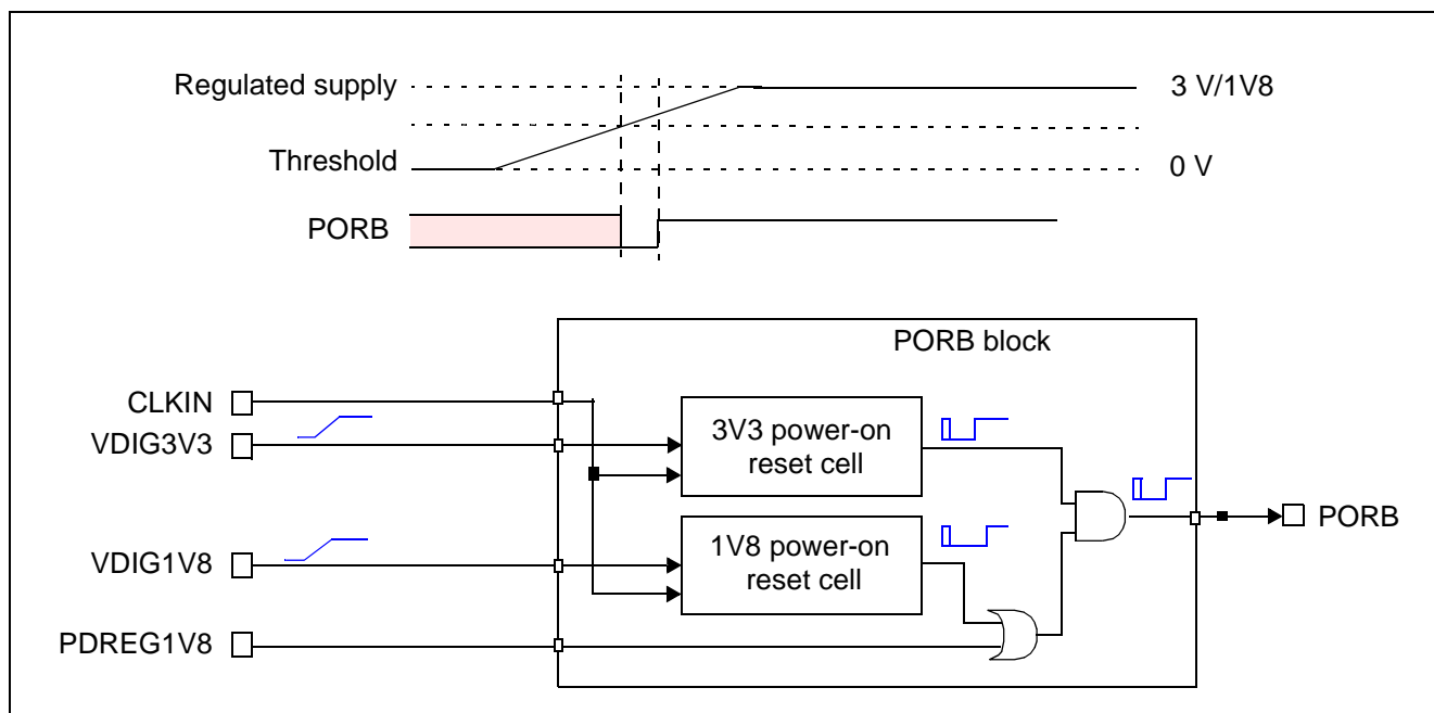
Figure 20: Power-on reset block
