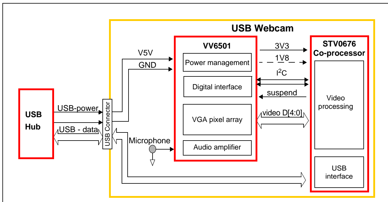
Figure 2: USB camera system using STV0676
