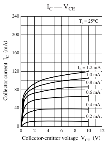
Characteristics charts of UNR921KJ
