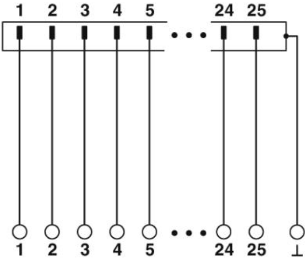
Circuit diagram
