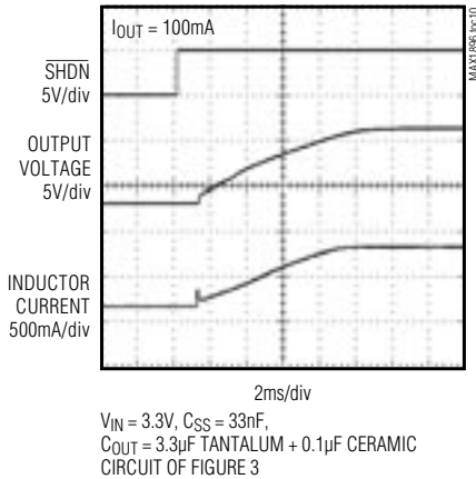
STARTUP WAVEFORM WITH SOFT-START
