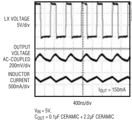
SWITCHING WAVEFORM
