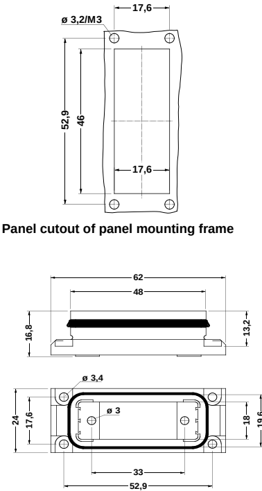
Dimensions: Panel mounting frame
