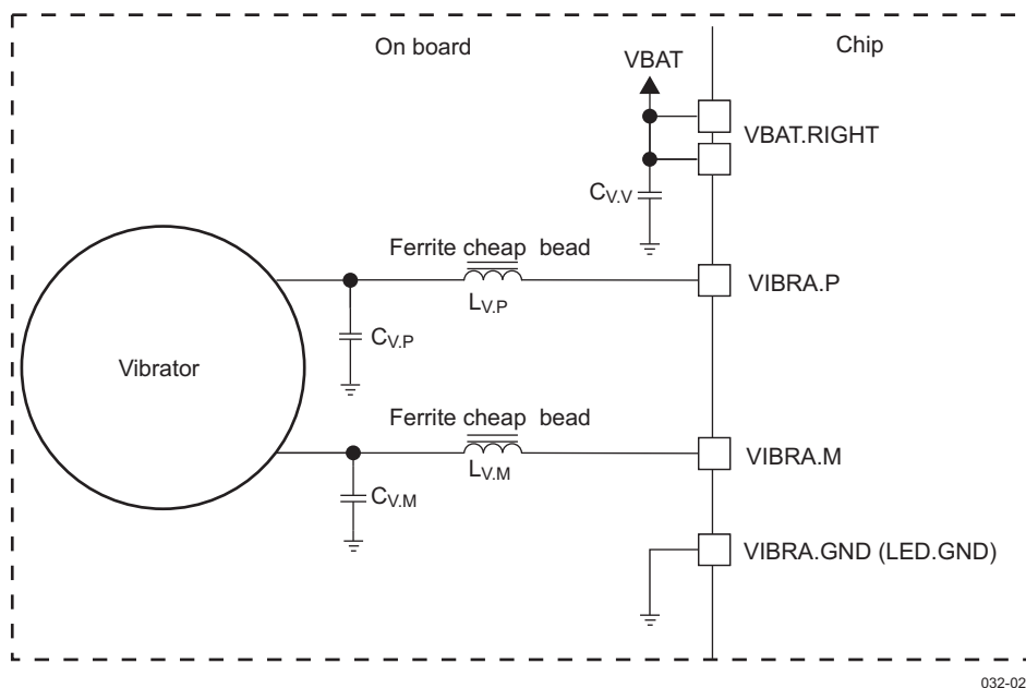
Figure 6-13. Vibrator H-Bridge
