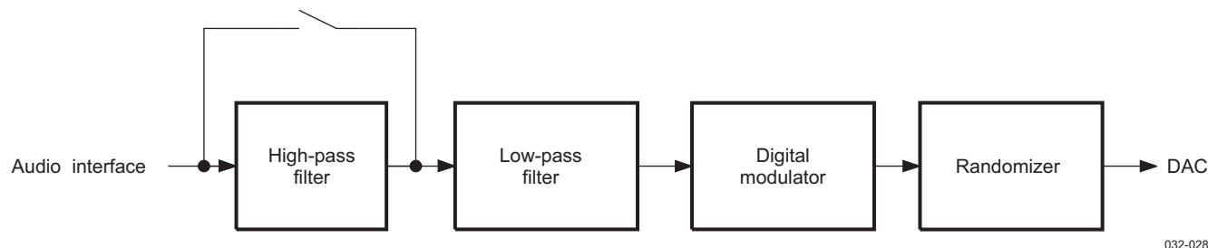
Figure 6-15. Digital Audio Filter Downlink Path Characteristics
