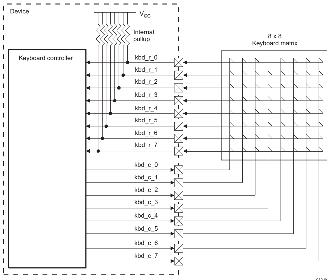
Figure 11-1. Keyboard Connection
