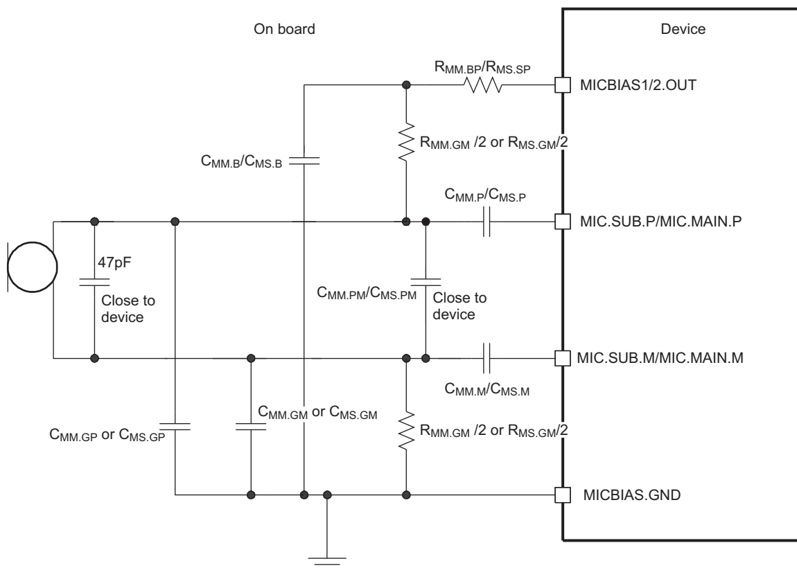
Figure 6-21. Analog Microphone Differential
