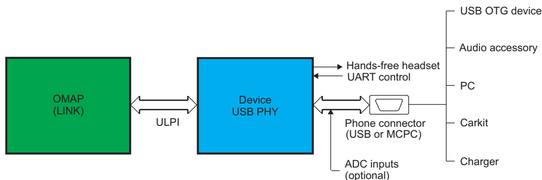
Figure 7-1. USB 2.0 PHY Overview
