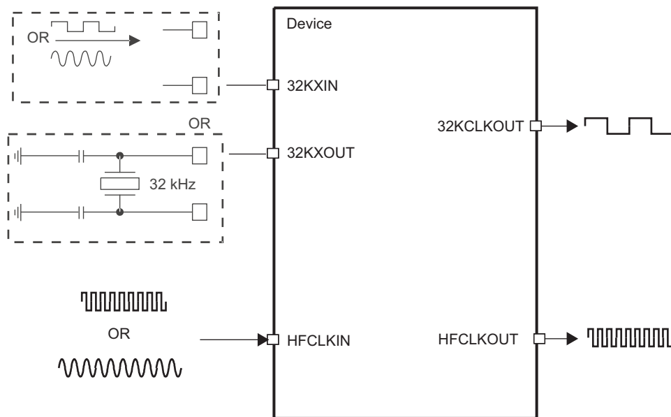
Figure 12-1. Clock Overview
