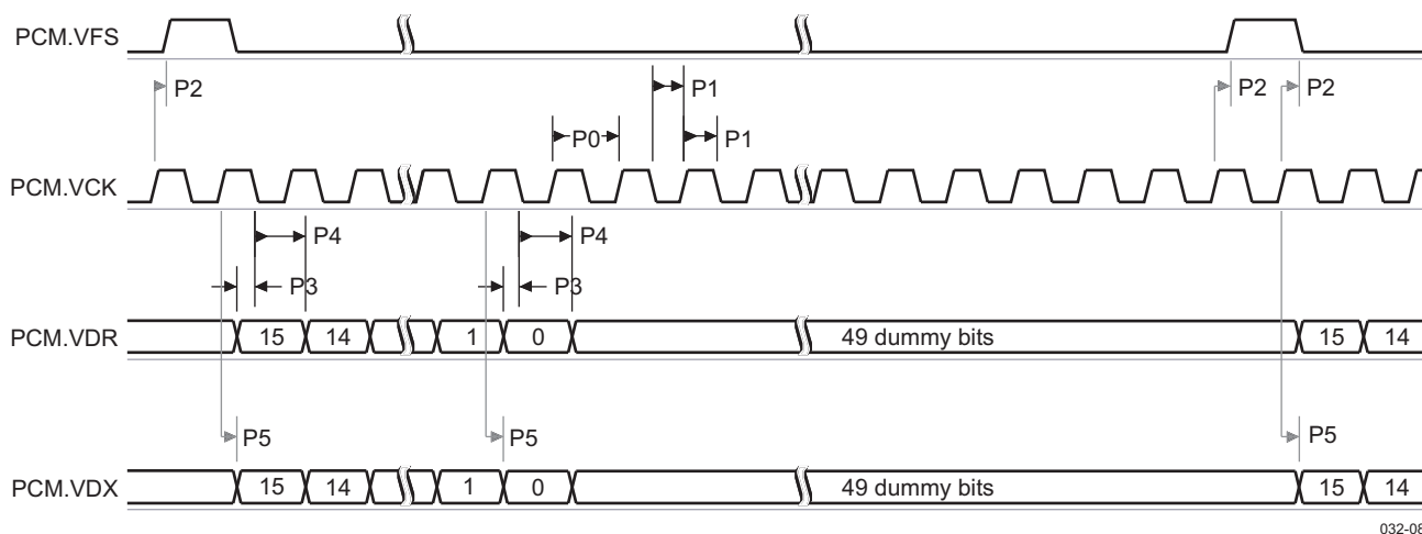
Figure 13-5. Voice/BT PCM Interface—Master Mode (Mode 1)
