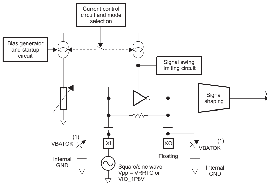
Figure 12-8. 32-kHz Oscillator Block Diagram Without Crystal Option 2
