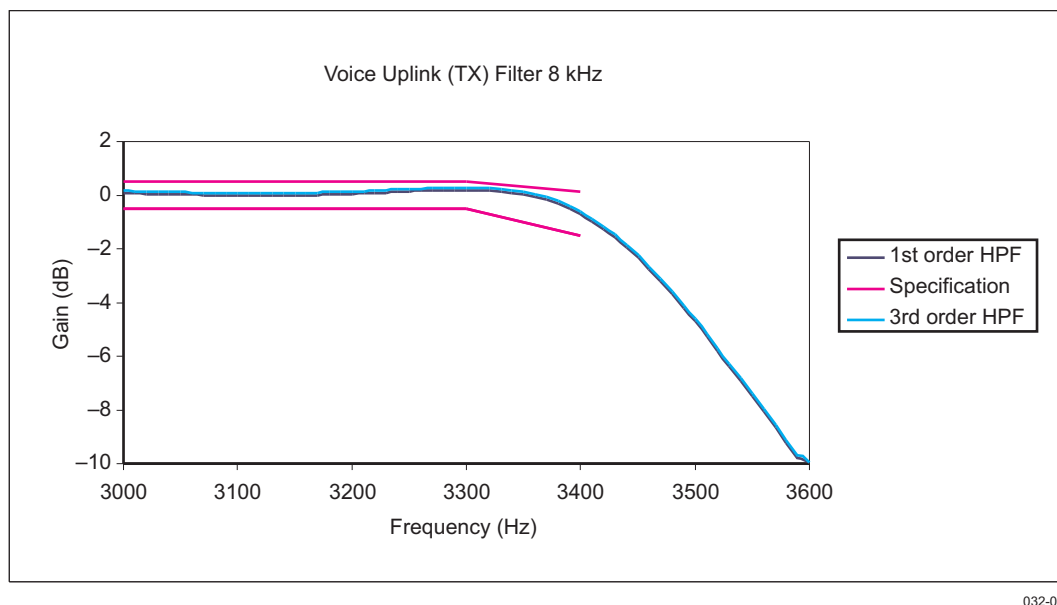
Figure 6-32. Voice Uplink Frequency Response With F_S = 8 kHz (Frequency Range 3000 to 3600 Hz)
