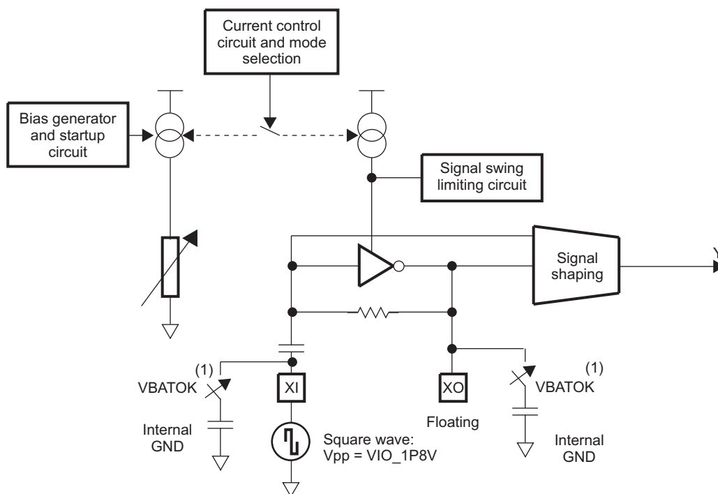
Figure 12-9. 32-kHz Oscillator in Bypass Mode Block Diagram Without Crystal Option 3
