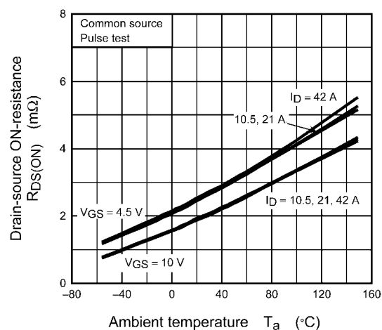
Fig. 8.6 R_{DS(ON)} - T_a
