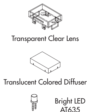
AT4177 Rectangular
