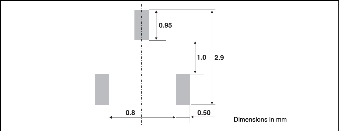
Figure 12. Footprint dimensions
