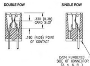
SECTIONS THROUGH CONTACT POSITION
