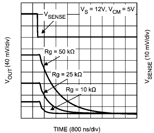
Settling time (fall)
