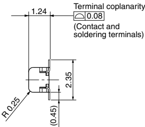
Dimension table (mm)
