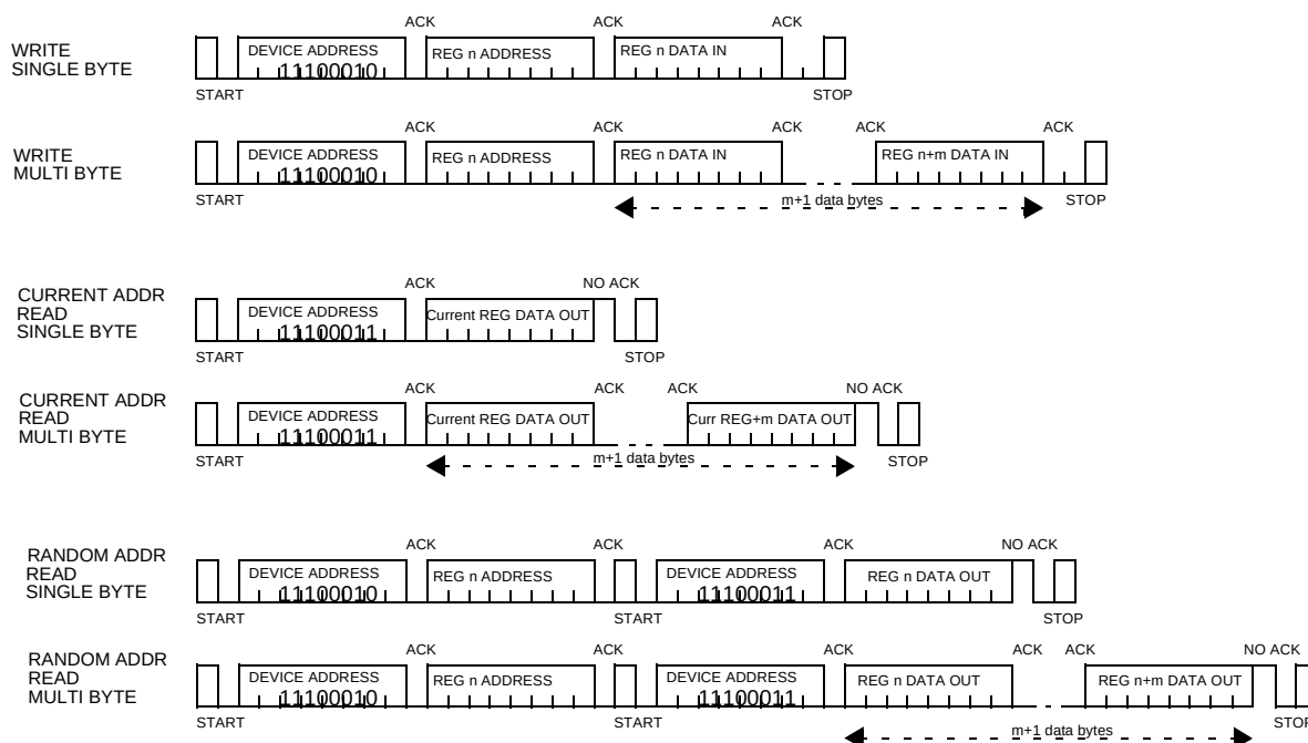
Figure 14. Control interface (I 2 C I/F) formats
