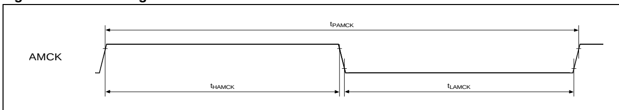
Figure 4. AMCK timing
