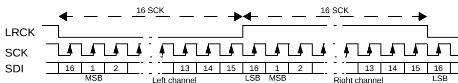
Figure 10. Audio interface (AU I/F) formats in I 2 S master and slave modes
