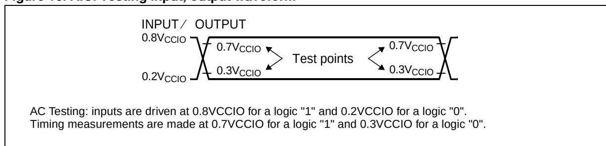
Figure 16. A.C. Testing input, output waveform
