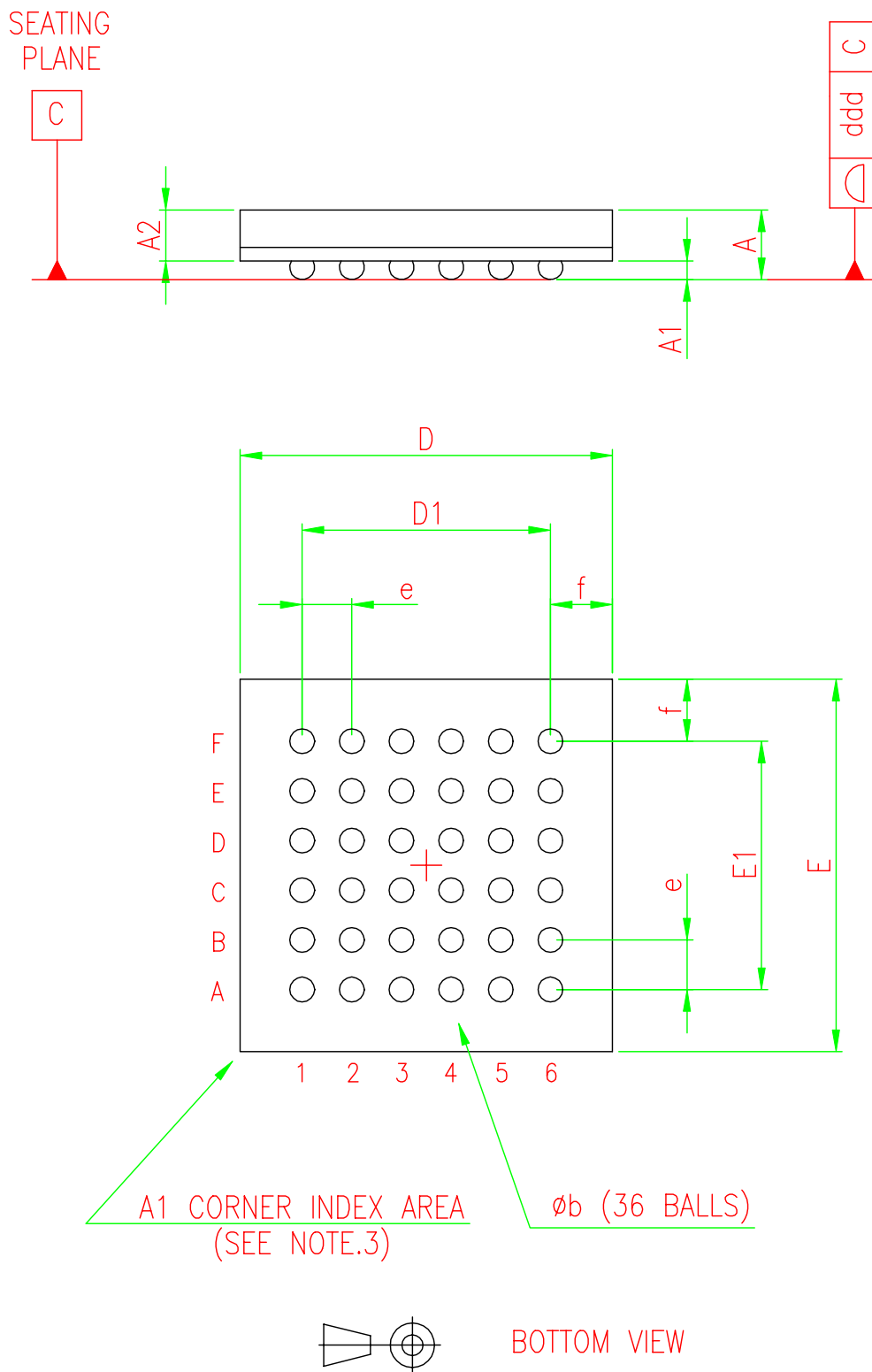
Figure 17. TFBGA36 drawing
