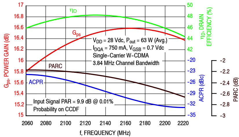
Figure 3. Single-Carrier Output Peak-to-Average Ratio Compression (PARC) Broadband Performance @ P_{out} = 63 \text{ Watts Avg.}
