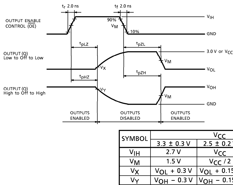
Fig.4 t_{pLZ} , t_{pHZ} , t_{pZL} , t_{pZH}
