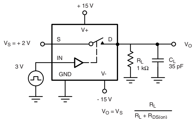
Figure 2. Switching Time
