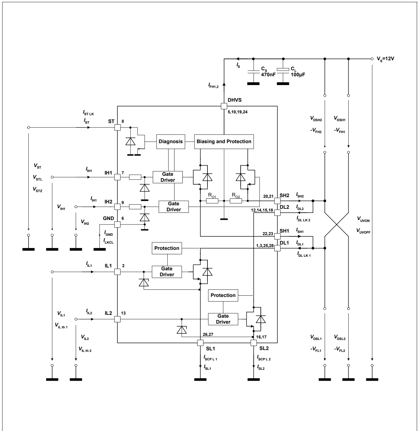
Figure 2 Terms BTM7741G
