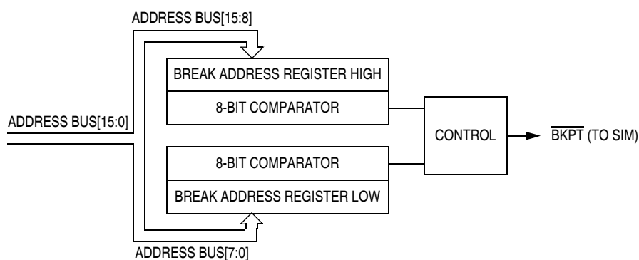
Figure 15-2. Break Module Block Diagram
