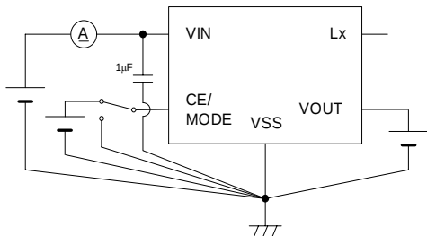
Circuit ⑤
