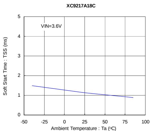
(9) Soft-start Time vs. Ambient Temperature
