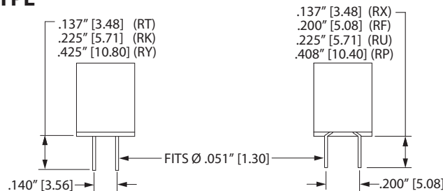
WIDE DIP SOLDER (RF, RX, RU, RP)
