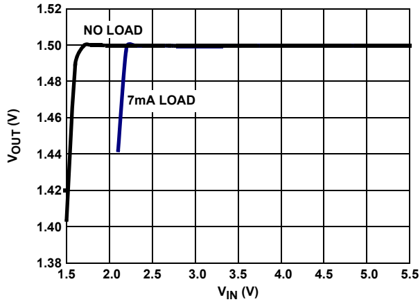
FIGURE 24. DROPOUT
