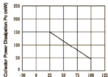
Fig.2 Collector Power Dissipation vs. Ambient Temperature
