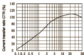
Fig.1 Current Transfer Ratio vs. Forward Current
