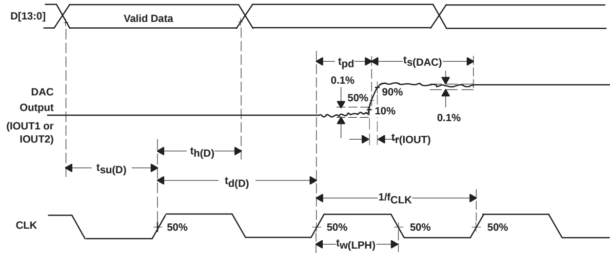
Figure 29. Timing Diagram
