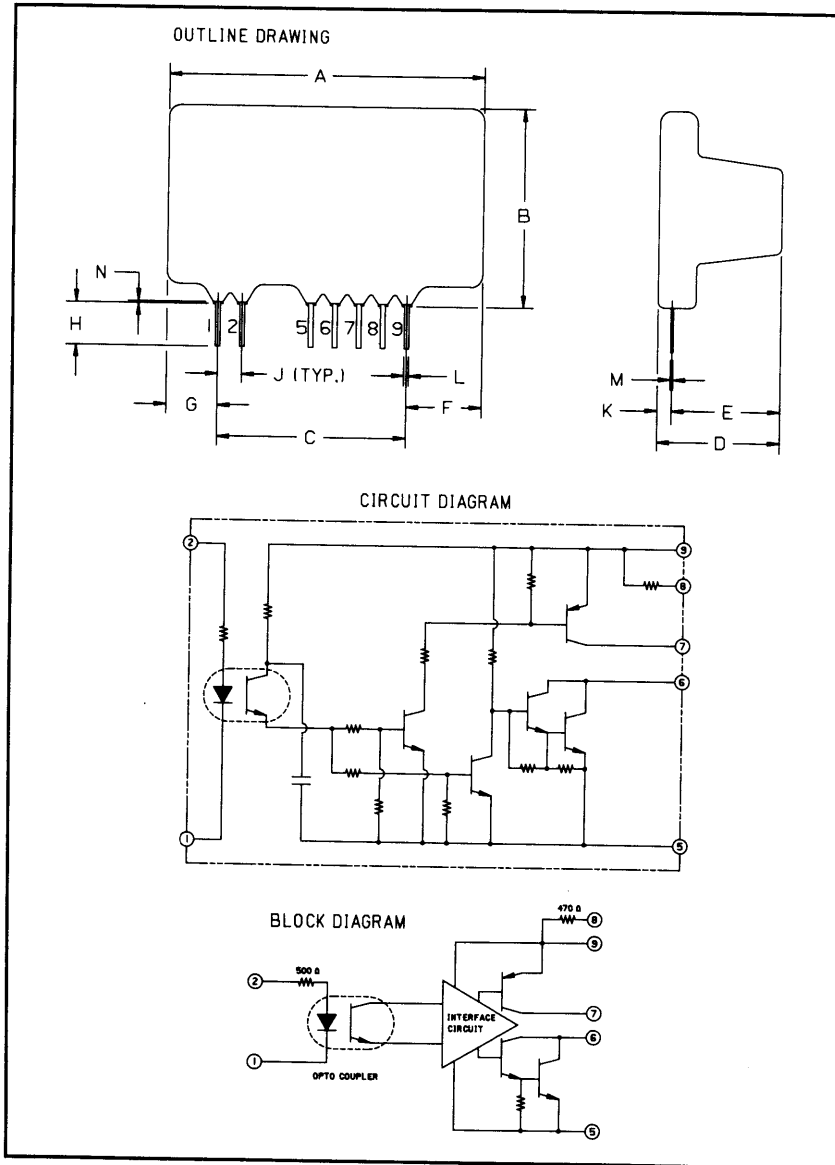
Outline Drawing
