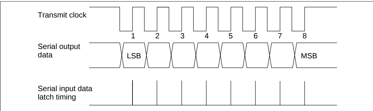
Figure 66 Serial Interface Output Timing
