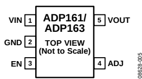
Figure 5. 5-Lead TSOT, Adjustable Output Pin Configuration, ADP161/ADP163
