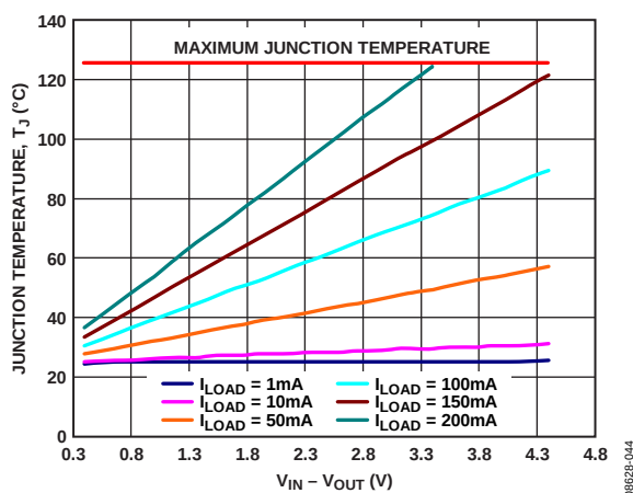
Figure 46. 100 mm² of PCB Copper, TSOT, T_A = 25^\circ\text{C}
