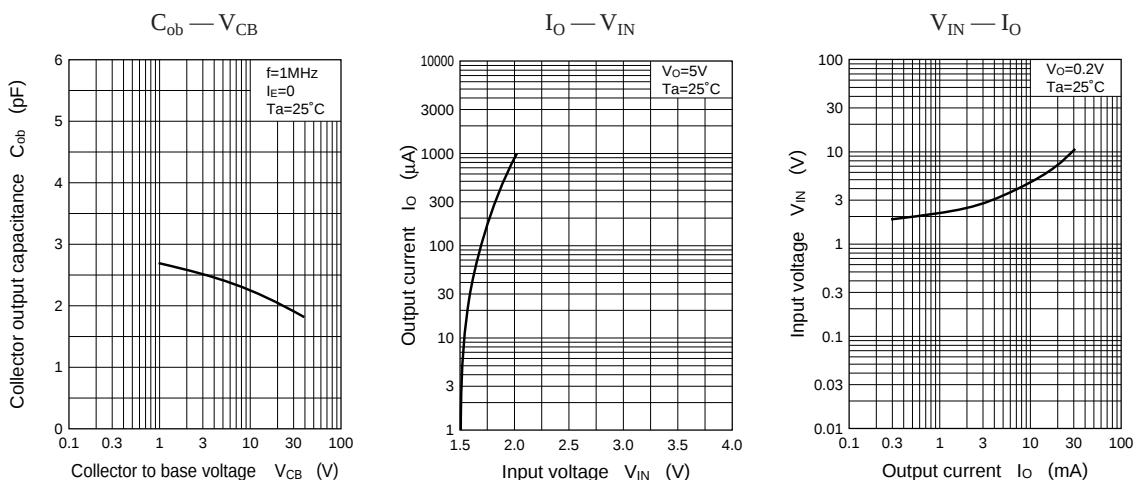
Characteristics charts of UN221F
