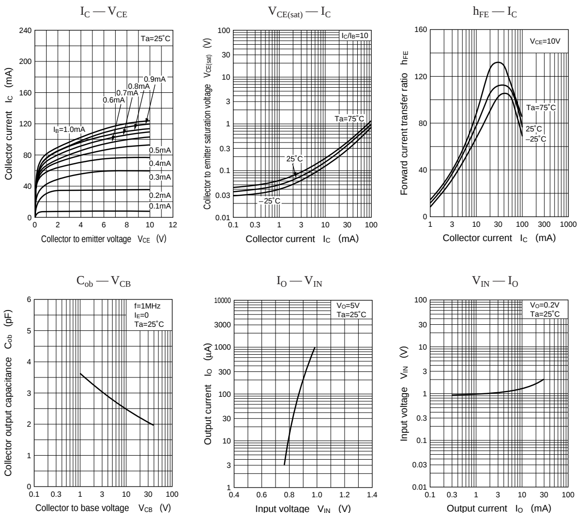
Characteristics charts of UN221F
