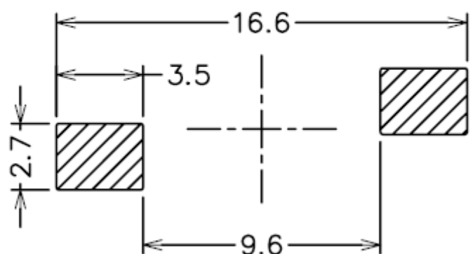
Soldering patterns
