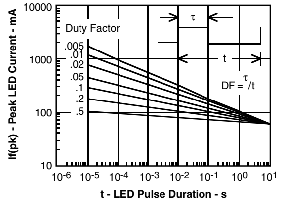
Figure 13. Peak LED current versus peak duration, Tau
