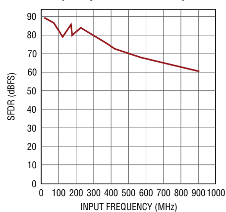
LTC2155-14: SFDR vs Input Frequency, -1\text{dBFS} , 170MSPs
