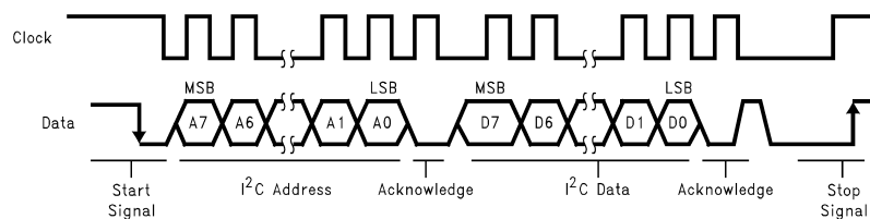
Figure 25. I²C Bus Format
